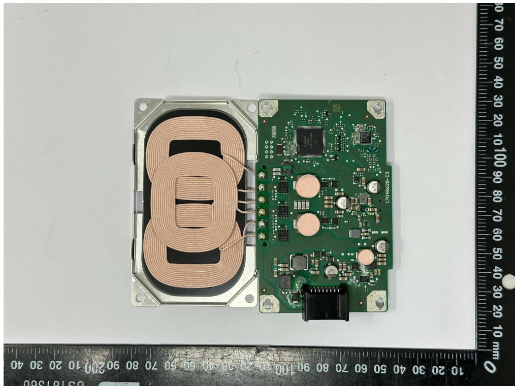
Figure 6 PCB and coil view
