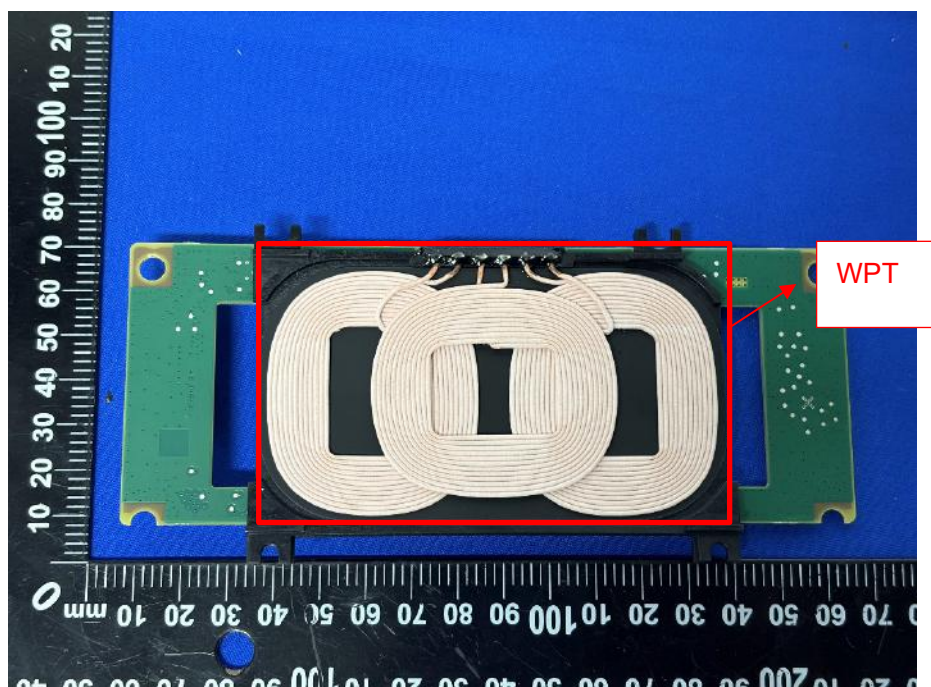
MAIN BOARD REAR VIEW
