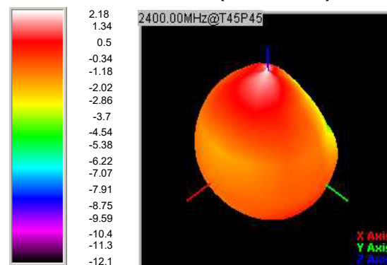
◎ 3D Gain Pattern (2400 MHz)
