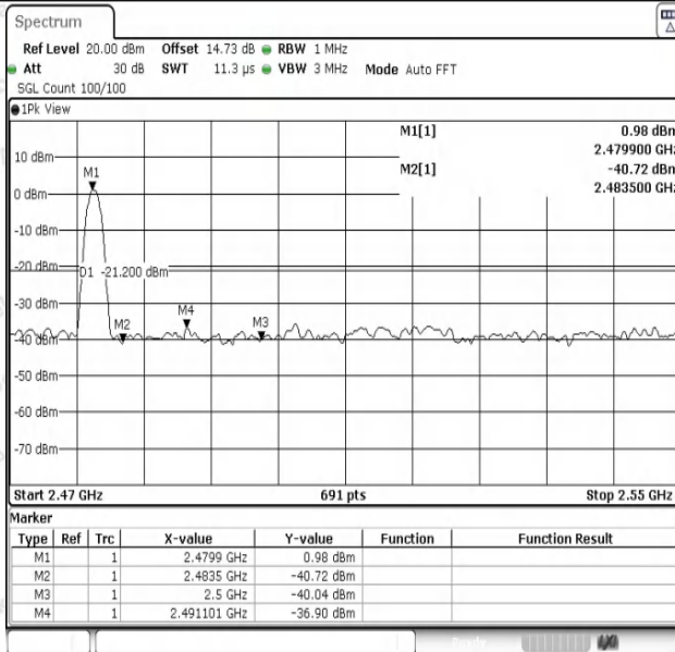
DH5-Ant1-2480-PASS
