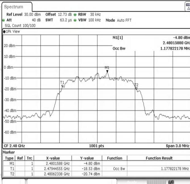
2DH5-Ant1-2480
