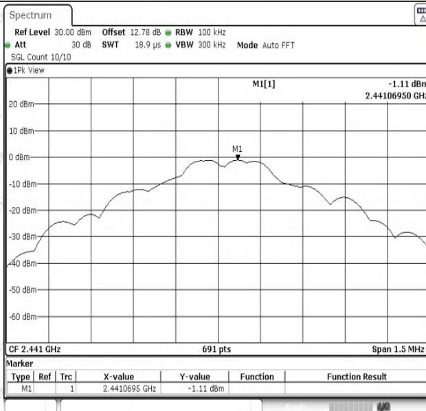
DH5-Ant1-2441-0~Reference-PASS
