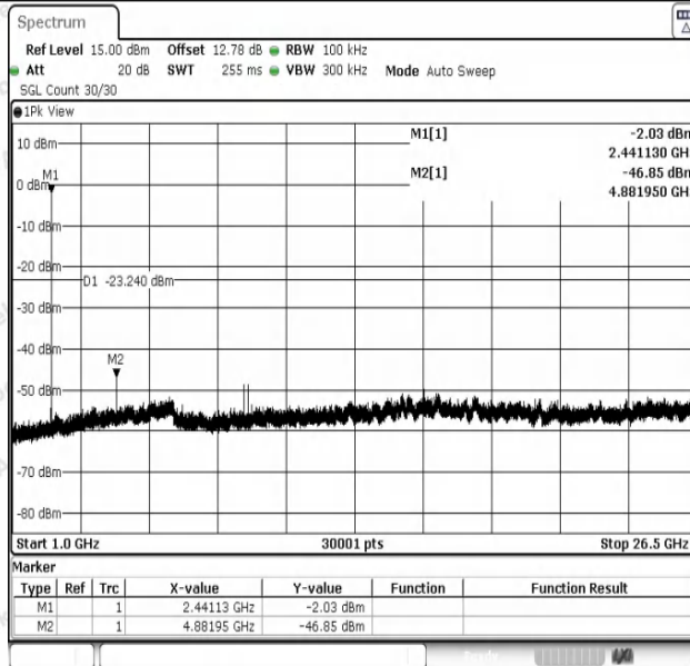
2DH5-Ant1-2441-1000~26500-PASS
