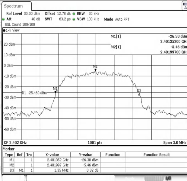
3DH5-Ant1-2402
