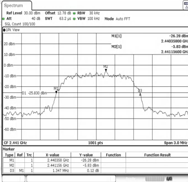
2DH5-Ant1-2441
