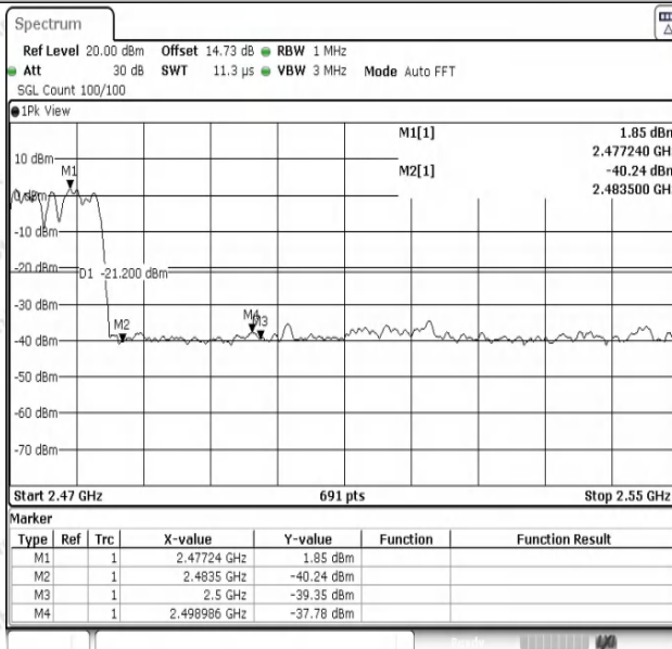
3DH5-Ant1-Hop_2480-PASS
