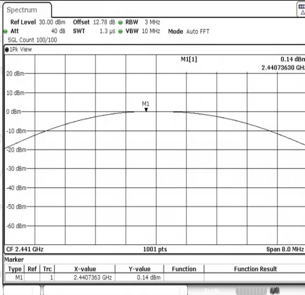
DH5-Ant1-2441-PASS
