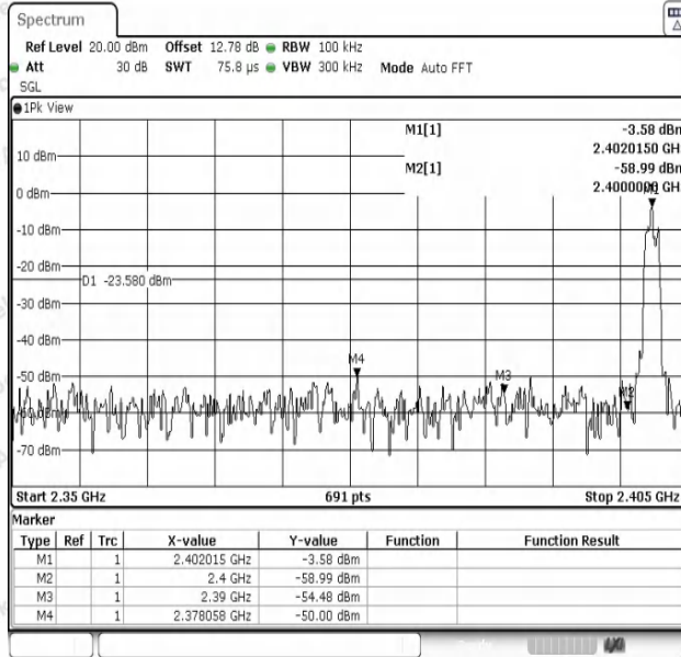
2DH5-Ant1-2402-PASS
