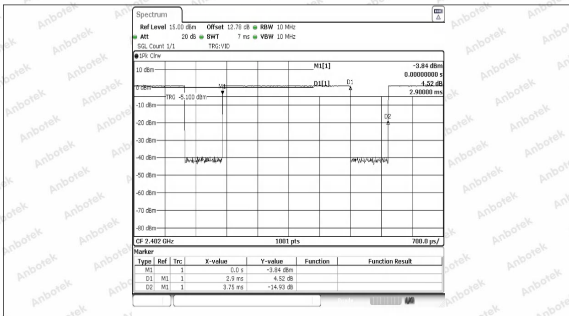
NTNV-DH5-Ant1-2402
