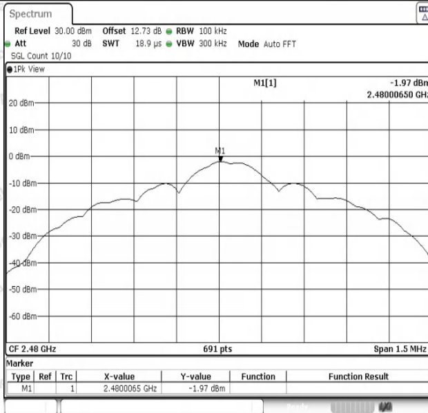
DH5-Ant1-2480-0~Reference-PASS
