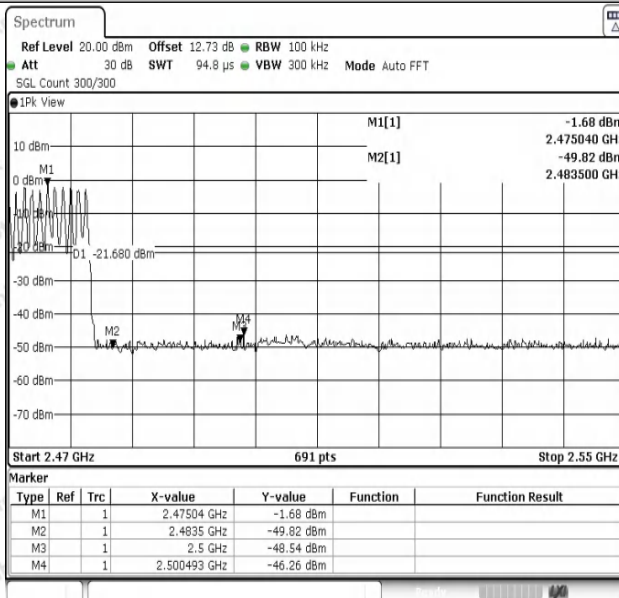
DH5-Ant1-Hop_2480-PASS
