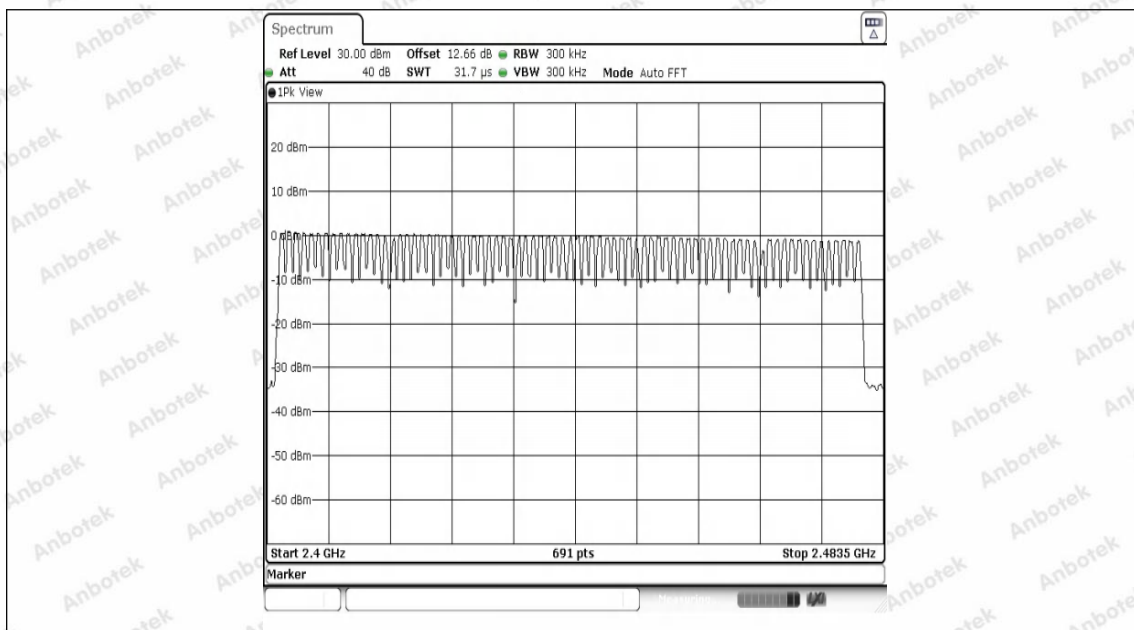
DH5-Ant1-Hop-PASS
