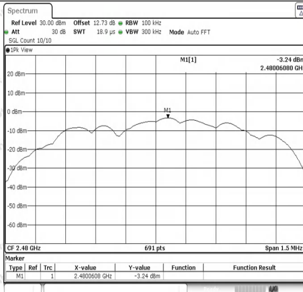
2DH5-Ant1-2480-0~Reference-PASS
