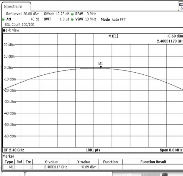
DH5-Ant1-2480-PASS
