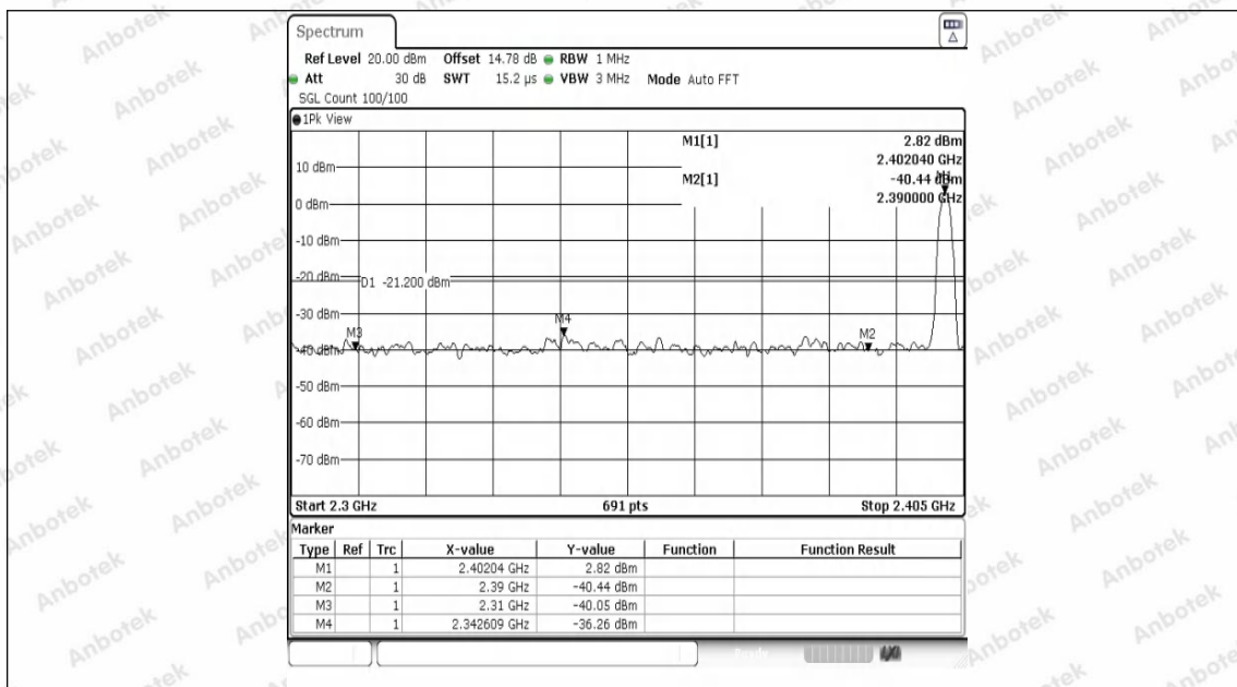
DH5-Ant1-2402-PASS
