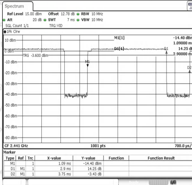
NTNV-2DH5-Ant1-2441
