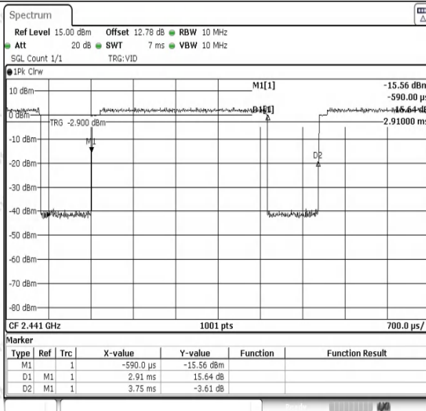
NTNV-3DH5-Ant1-2441
