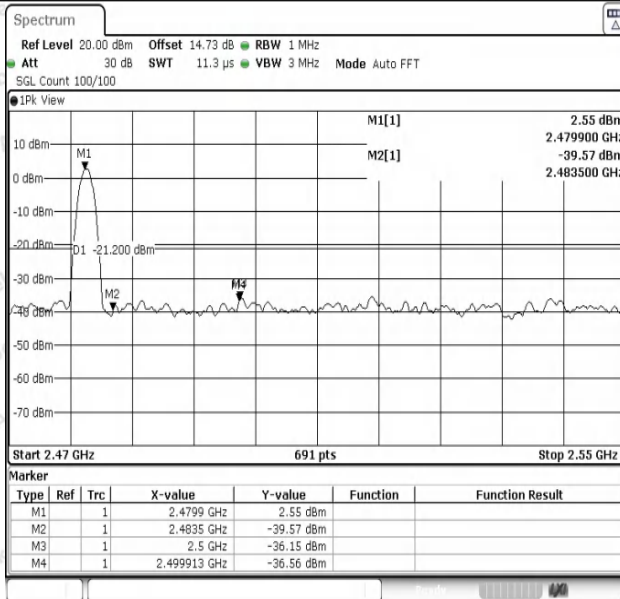
2DH5-Ant1-2480-PASS
