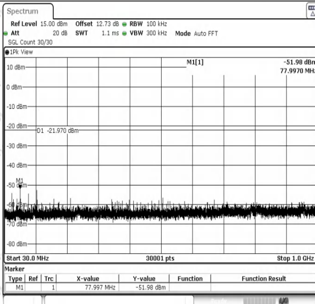
DH5-Ant1-2480-30~1000-PASS
