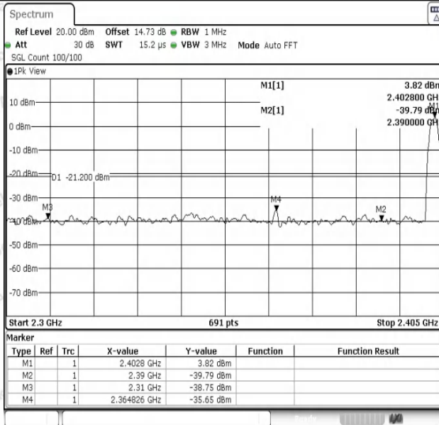
2DH5-Ant1-Hop_2402-PASS
