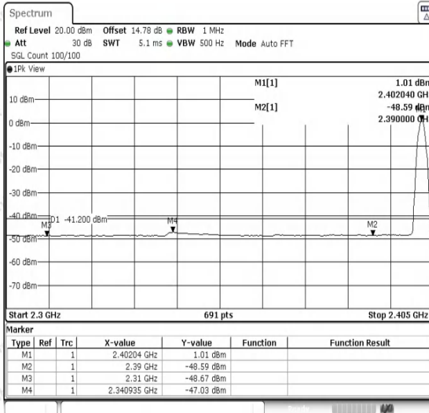
3DH5-Ant1-2402-PASS
