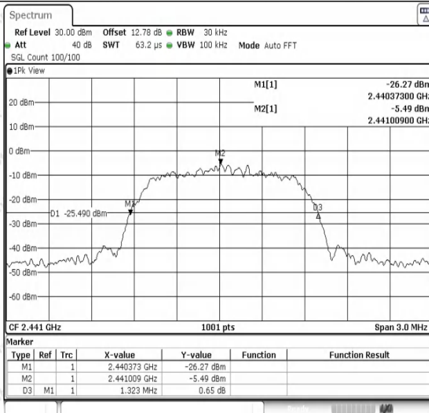
3DH5-Ant1-2441
