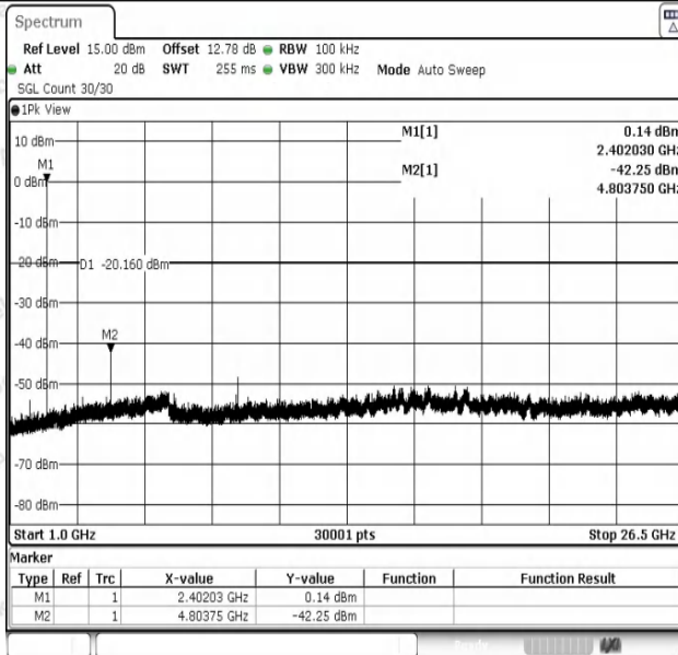
DH5-Ant1-2402-1000~26500-PASS
