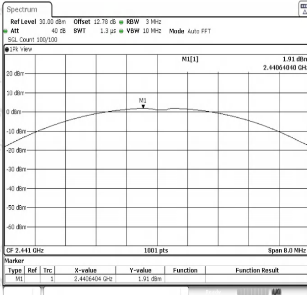
2DH5-Ant1-2441-PASS
