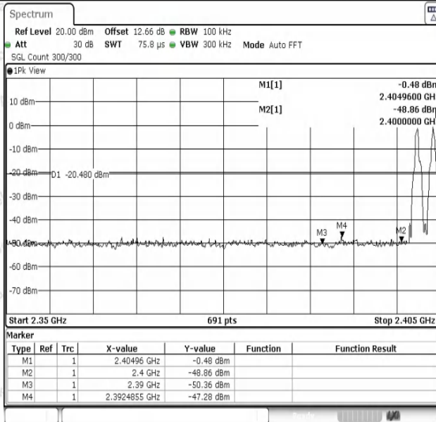
DH5-Ant1-Hop_2402-PASS
