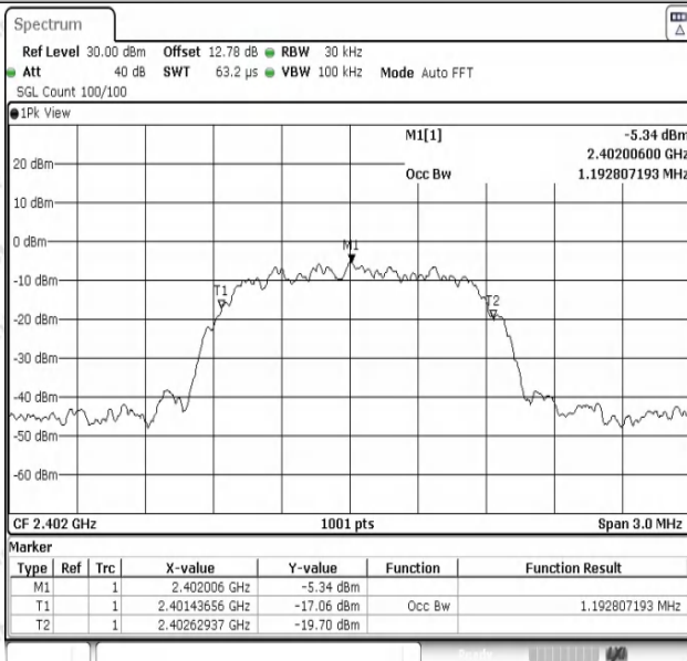
2DH5-Ant1-2402
