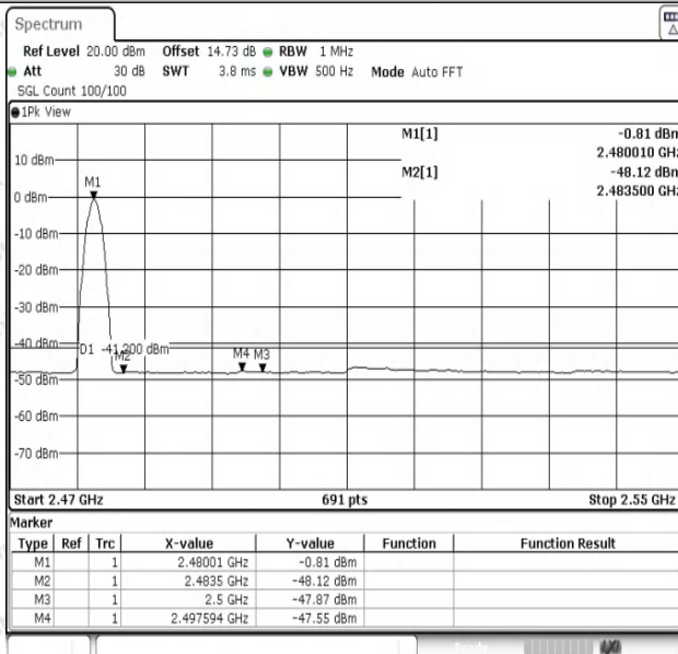
3DH5-Ant1-2480-PASS
