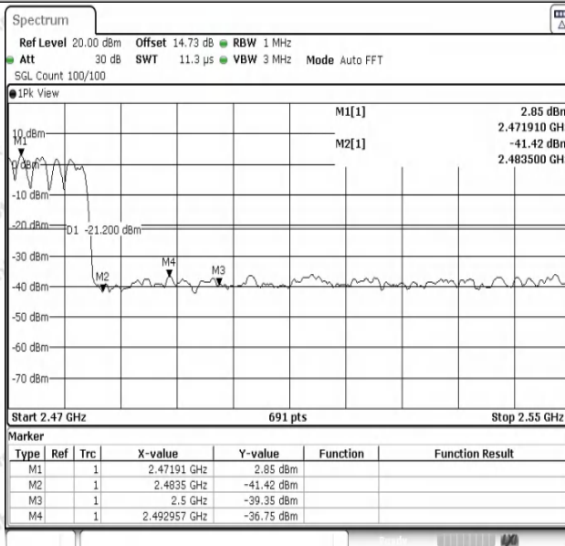
2DH5-Ant1-Hop_2480-PASS
