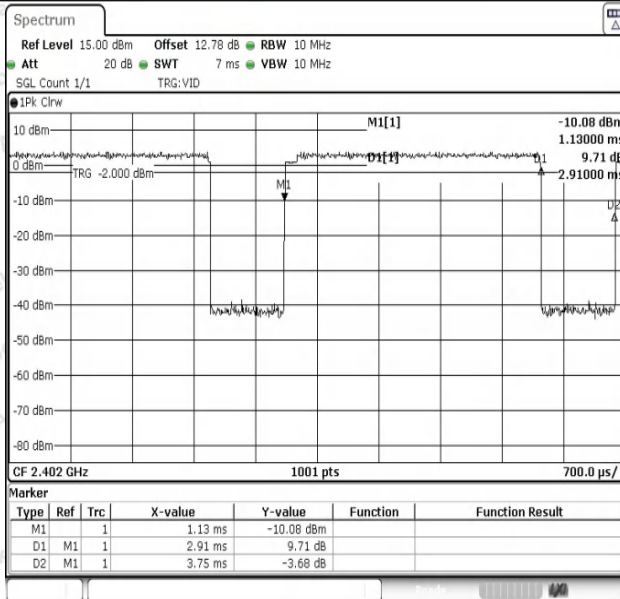
NTNV-3DH5-Ant1-2402
