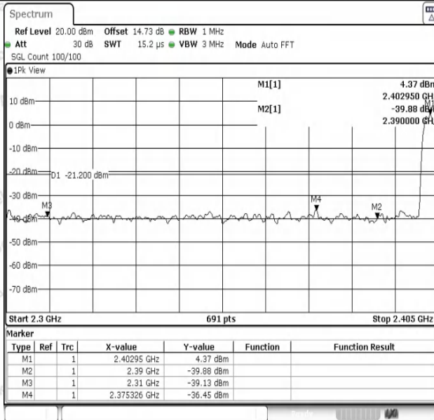
3DH5-Ant1-Hop_2402-PASS
