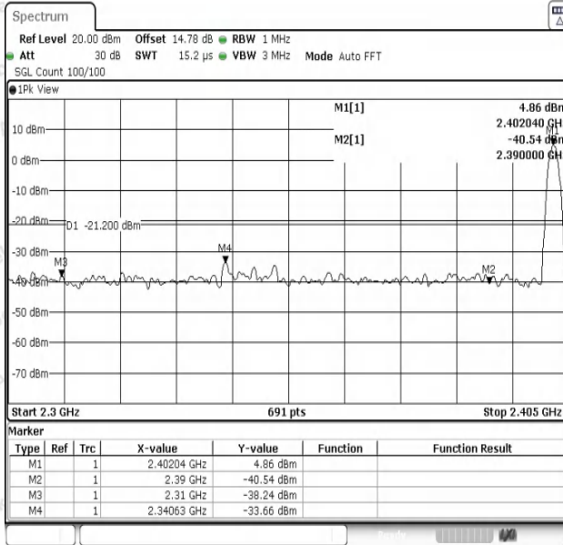
3DH5-Ant1-2402-PASS
