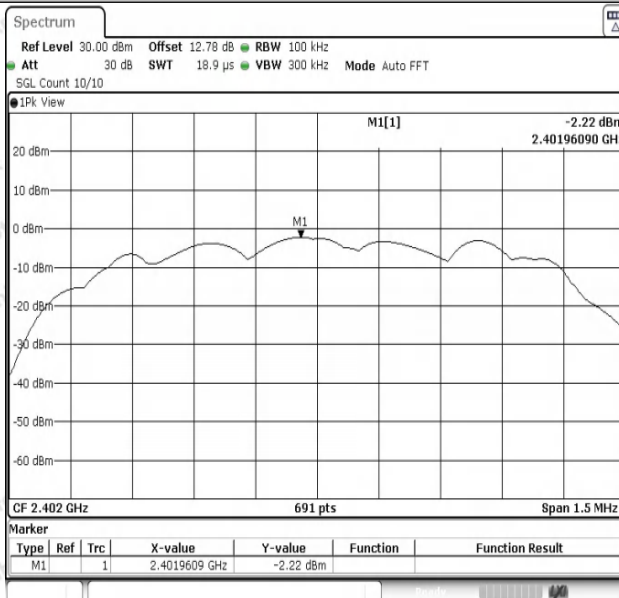
2DH5-Ant1-2402-0~Reference-PASS
