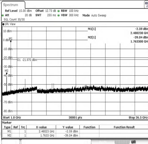
DH5-Ant1-2480-1000~26500-PASS
