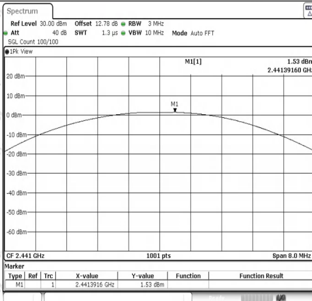
2DH5-Ant1-2441-PASS
