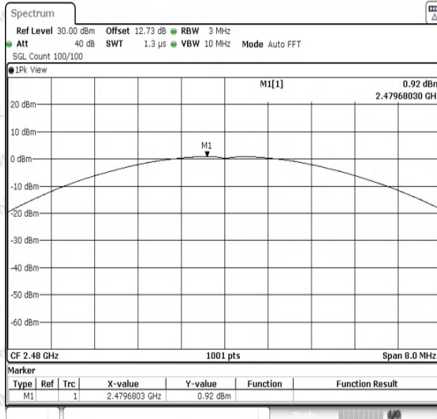
3DH5-Ant1-2480-PASS
