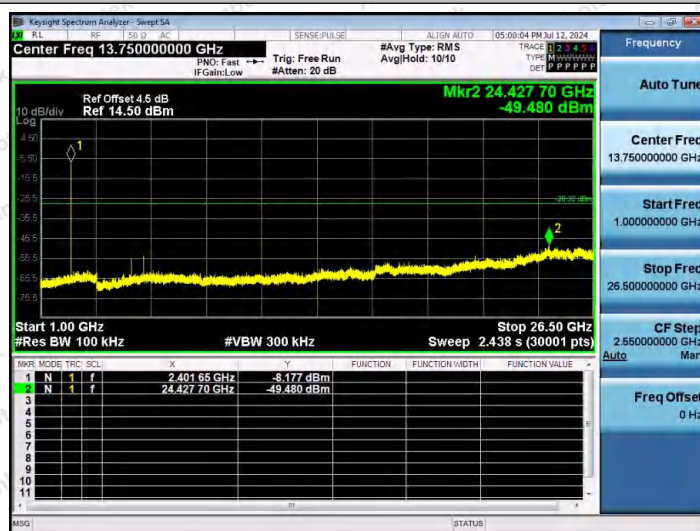
DH5-Ant1-2402-1000~26500-PASS
