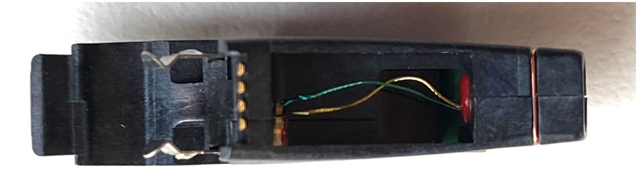
Hearing Aid with Left Antenna, Bottom View
