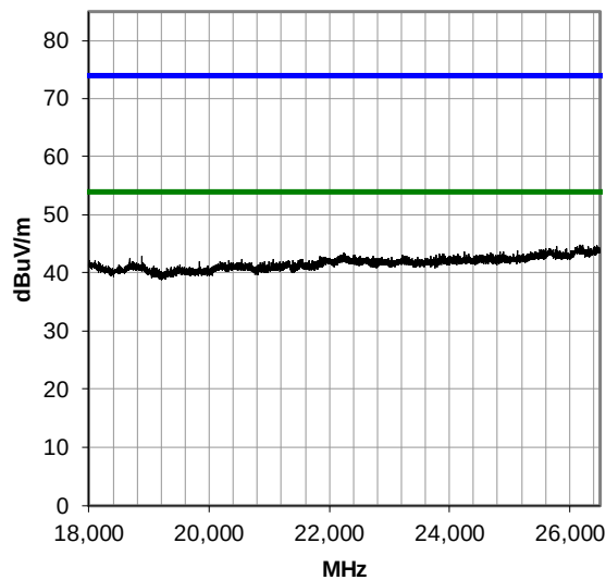
18000-26500 MHz, Ch. 0
