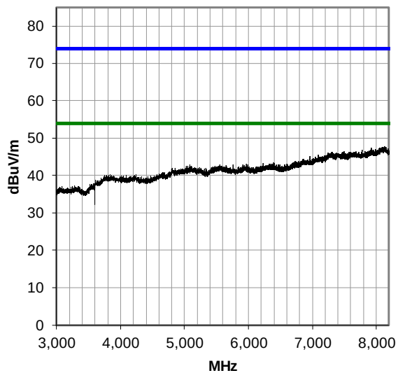
3000-8200 MHz, Ch. 39
