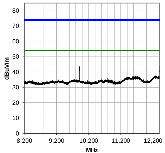
8200-12400 MHz, Ch. 39
