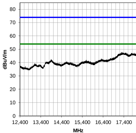
12400-18000 MHz, Ch. 0
