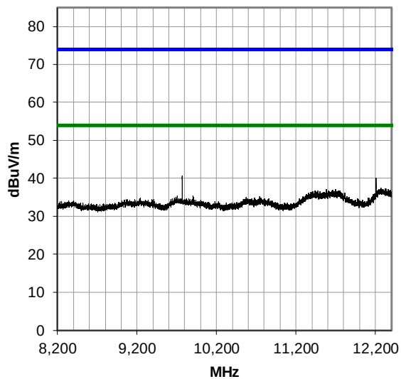
8200-12400 MHz, Ch. 20
