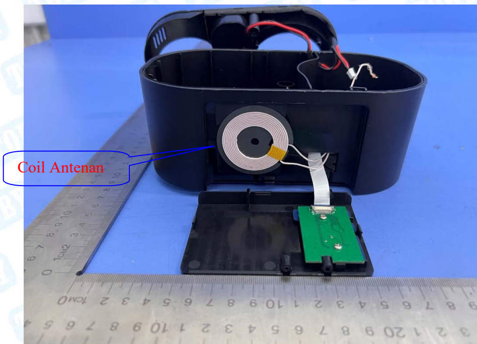
Photo 8 Internal of EUT
