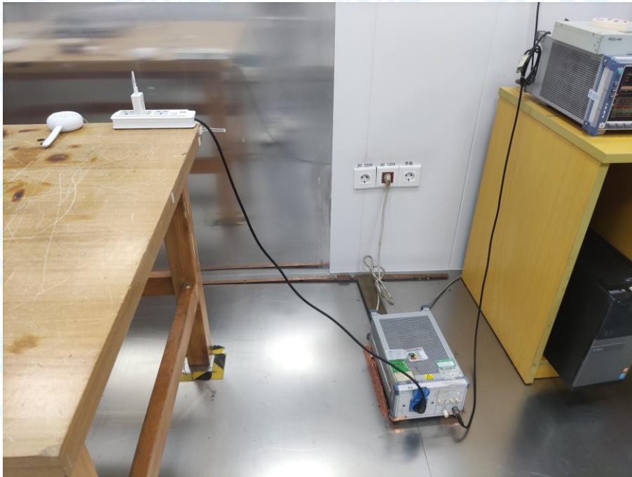
Photo of Setup for Conducted Emission
