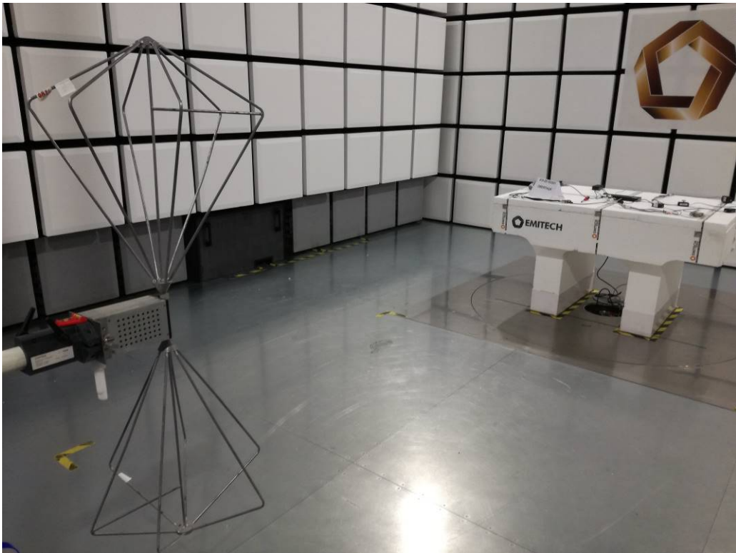
TEST SETUP PHOTO(S) – 30MHZ < FOR FREQ < 200MHZ
