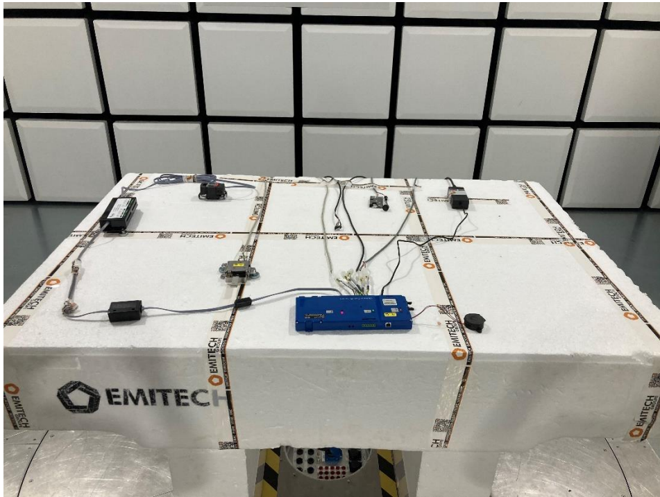
TEST SETUP PHOTO(S) -TX MODE – FOR FREQ <30MHZ
