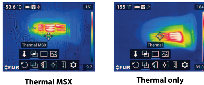
Figure 11.1 Thermal MSX image on left shows the detail from the digital camera image superimposed on the thermal image. Image on right shows the thermal only version.
