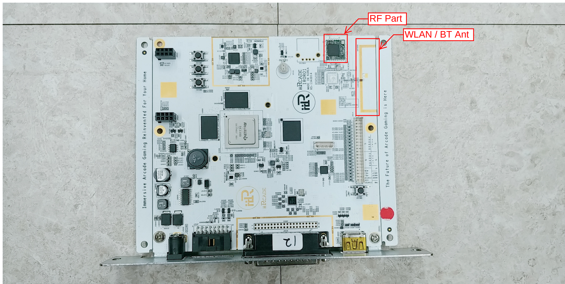
[Main board Top]
