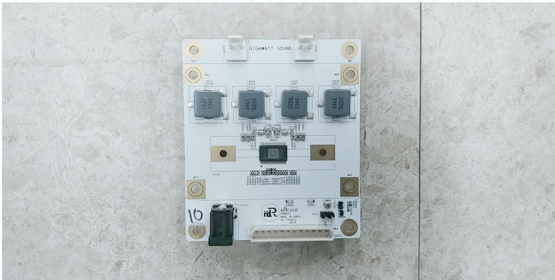
[Sub board1 Top]
