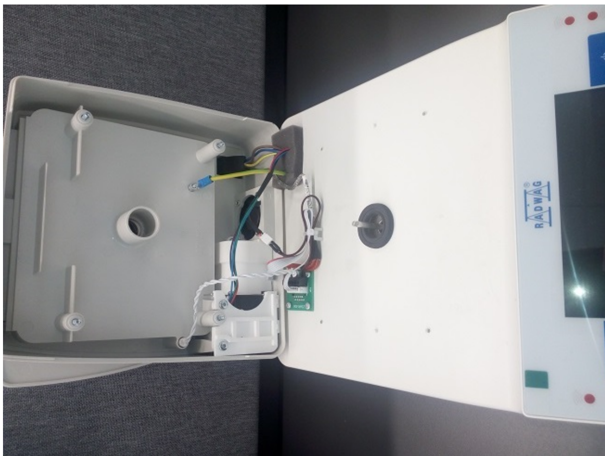
A cooling chamber under the weighing pan
