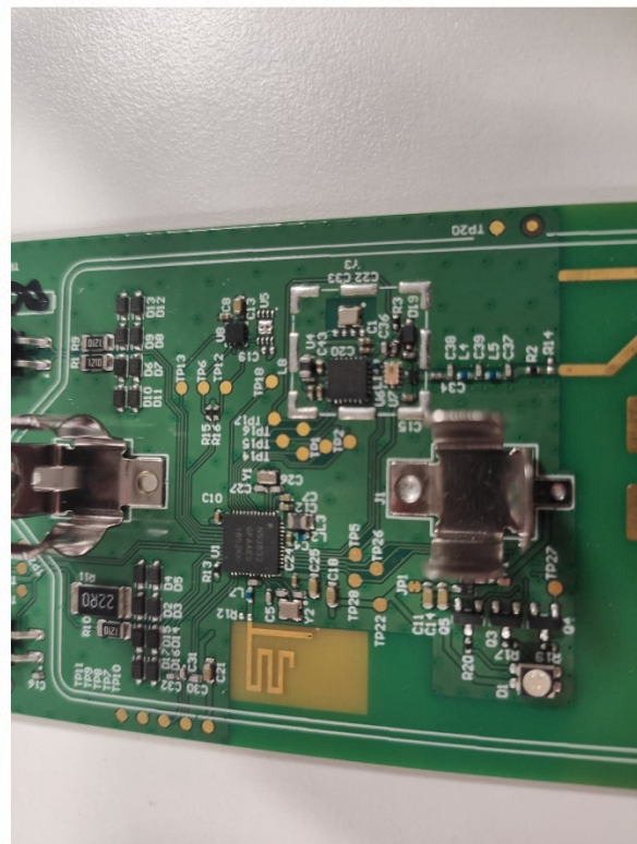
RF-Module Without Shielding
