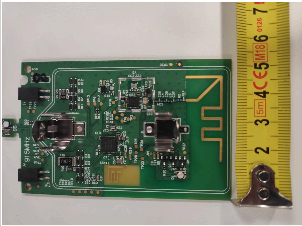
PCB Without Shielding View
