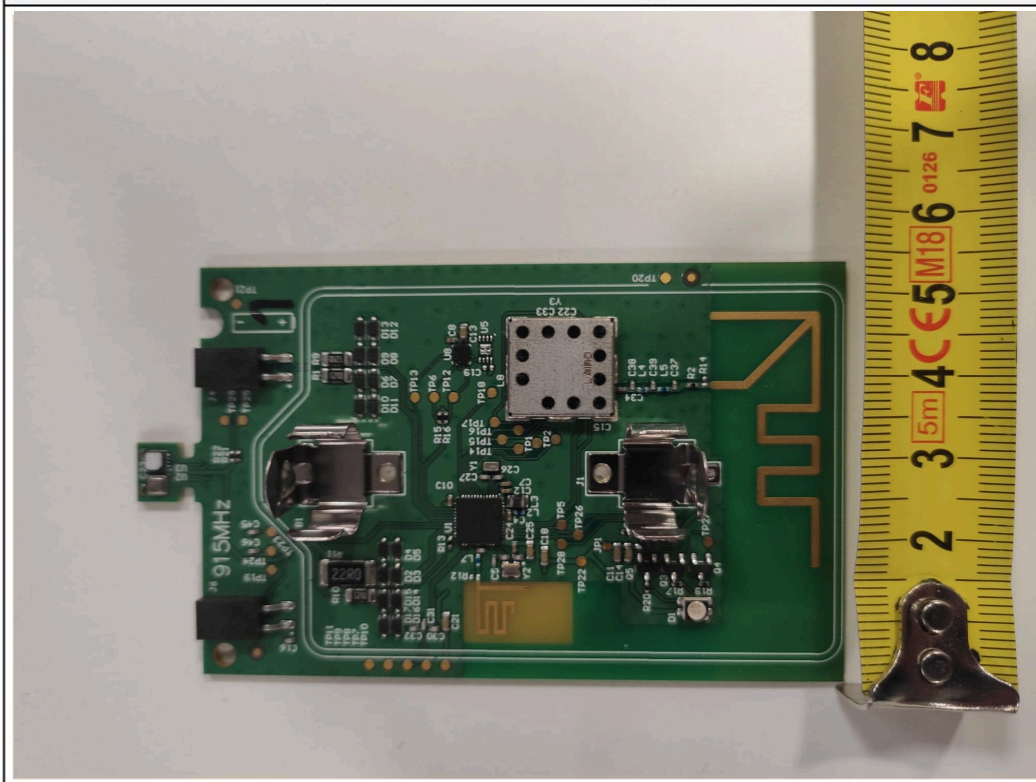
PCB Top View Without Potting Compound
