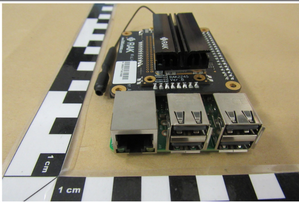
AE: LoRa Gateway View B
