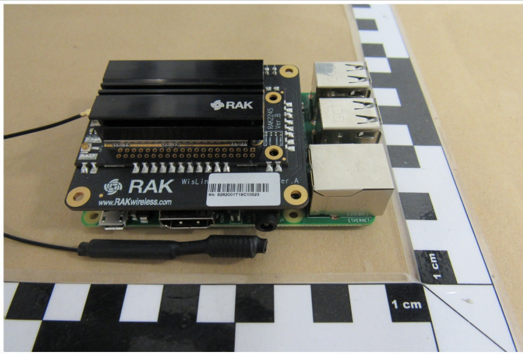
AE: LoRa Gateway View A
