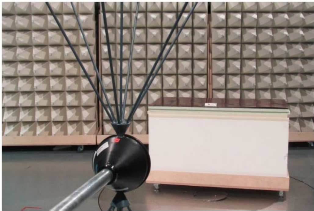
Radiated Setup View A
