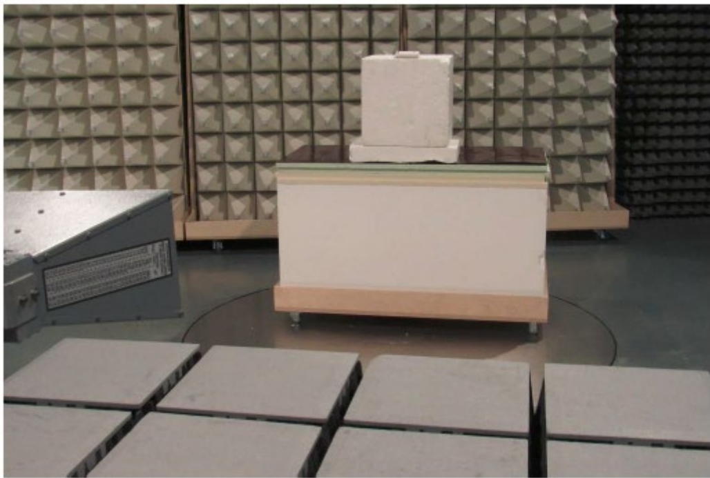
Radiated Setup View C
