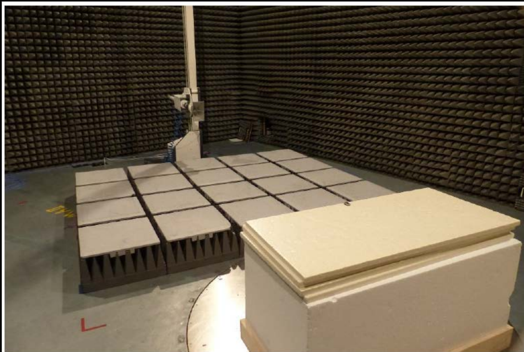
Test Setup EUT Configuration 1 1000-13000MHz
