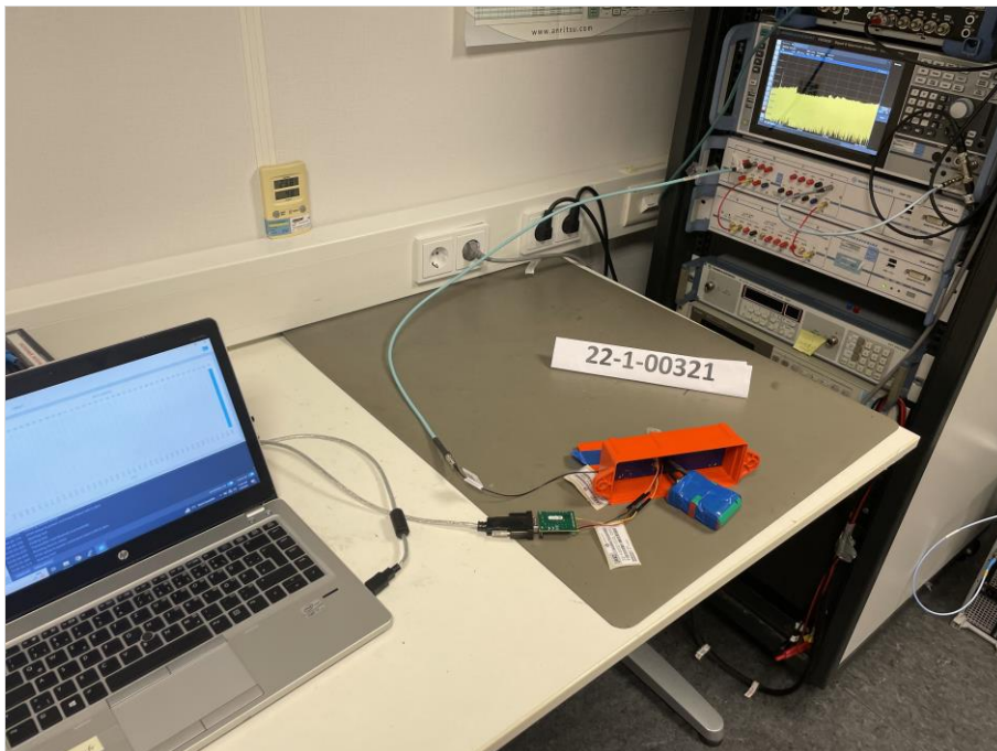
Photograph 6: EUT setup conducted measurement, overview
