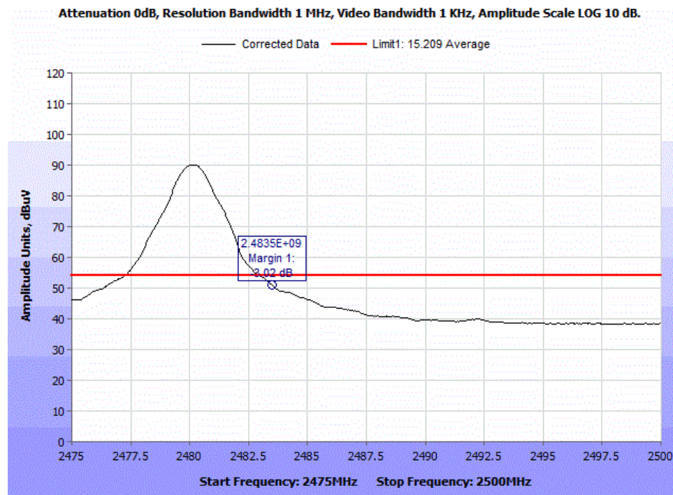
Radiated BandEdge, High Channel, 2480MHz, Average, H
