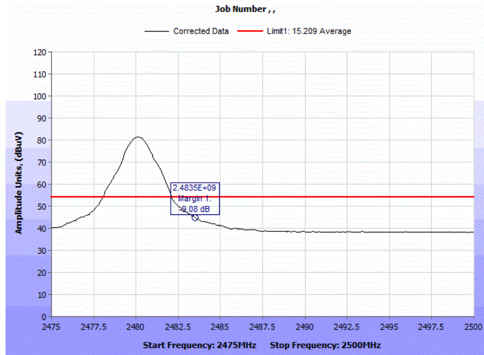
Radiated BandEdge, High Channel, 2480MHz, Average, V
