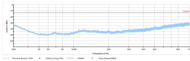
Plot #31 Radiated Emissions: 30 MHz – 1GHz
