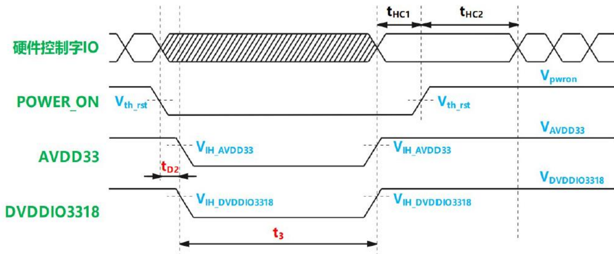
Figure 9-2 Power-off sequence
