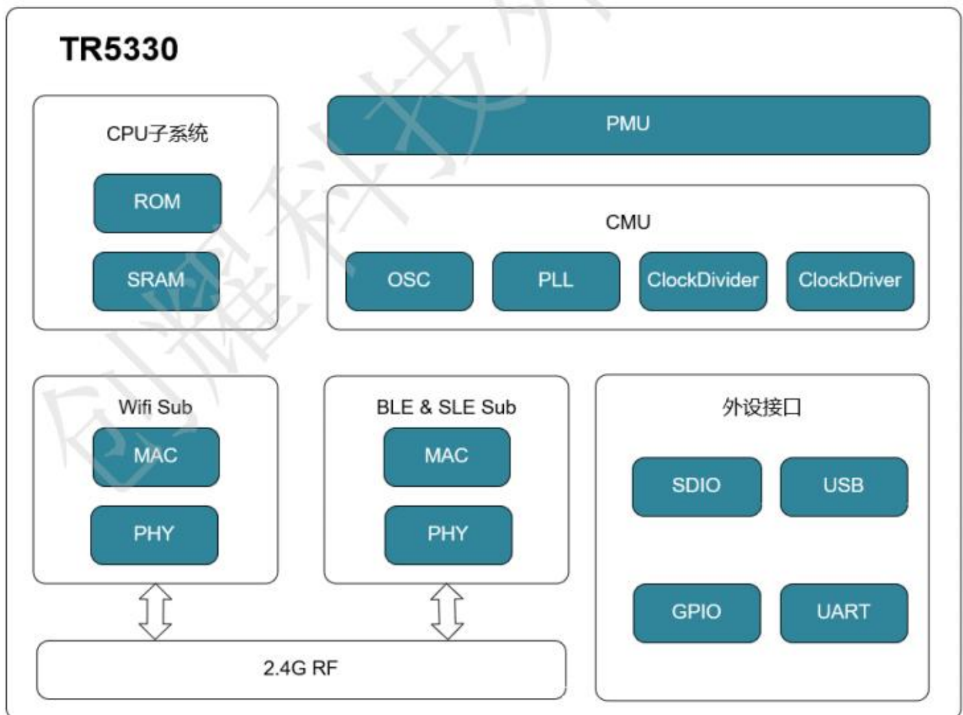
Figure 5-1 Hardware diagram of the FLC5330XSA-A
