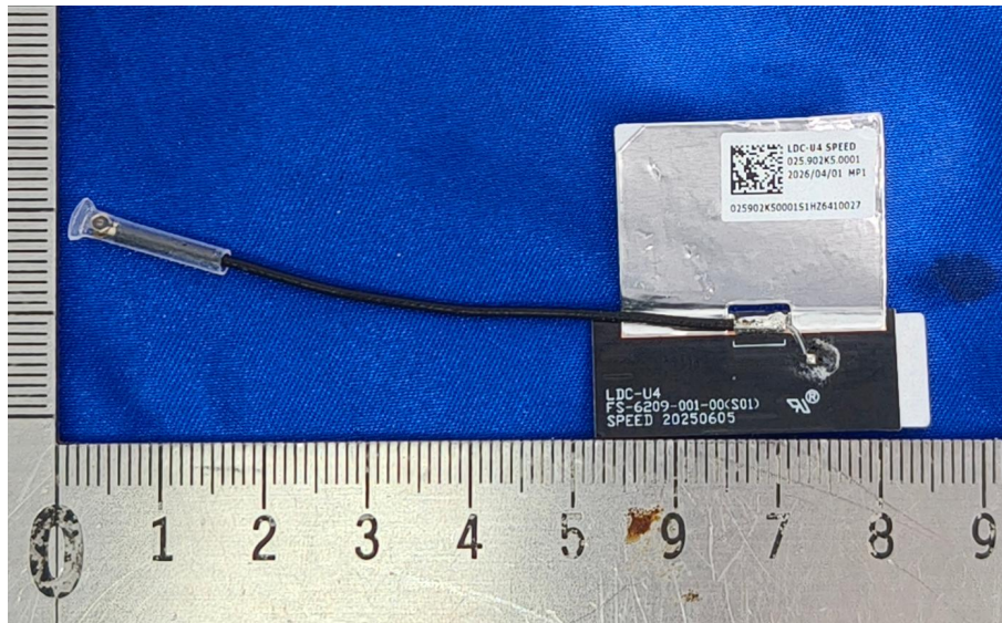
Ant3: Y4RYM0MA0BA
