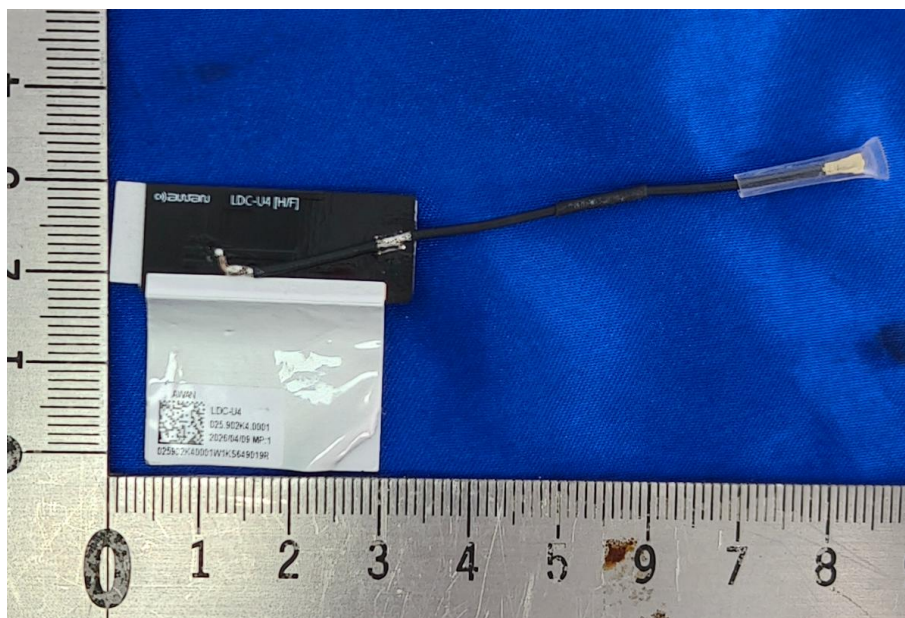
Ant1: AWAN
