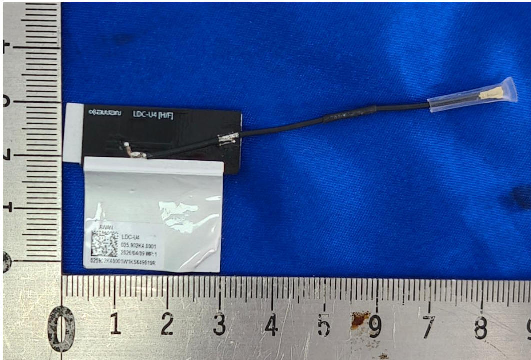
Ant2: SPEEDWIRE
