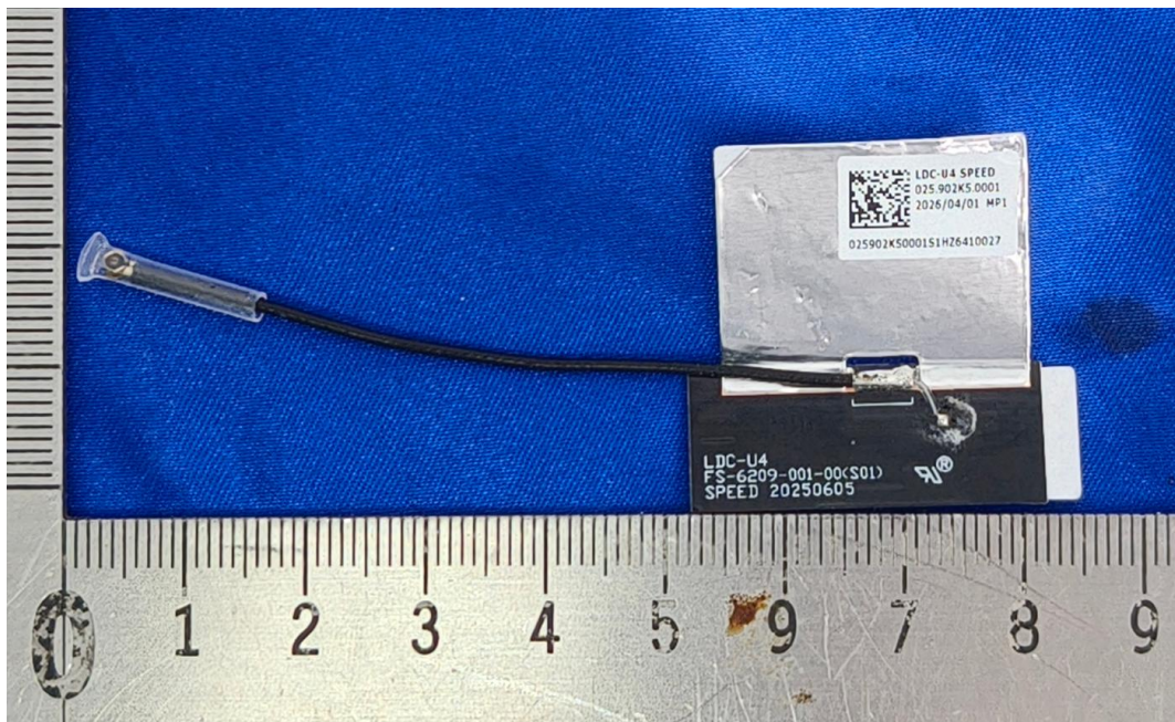
Ant2: SPEEDWIRE
