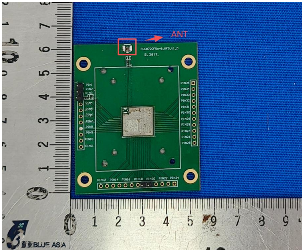
Development board
