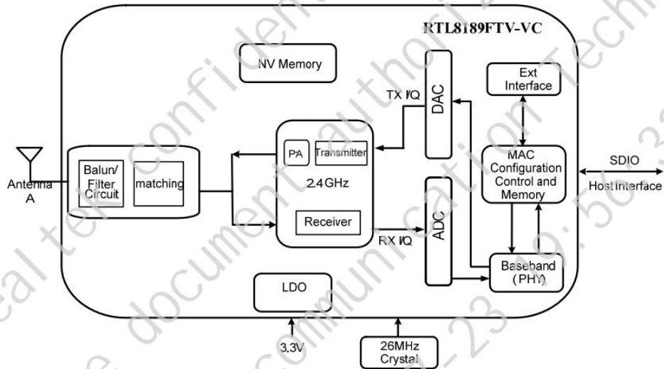
Figure 1FLW8189FSA7-A Hardware Block Diagram
