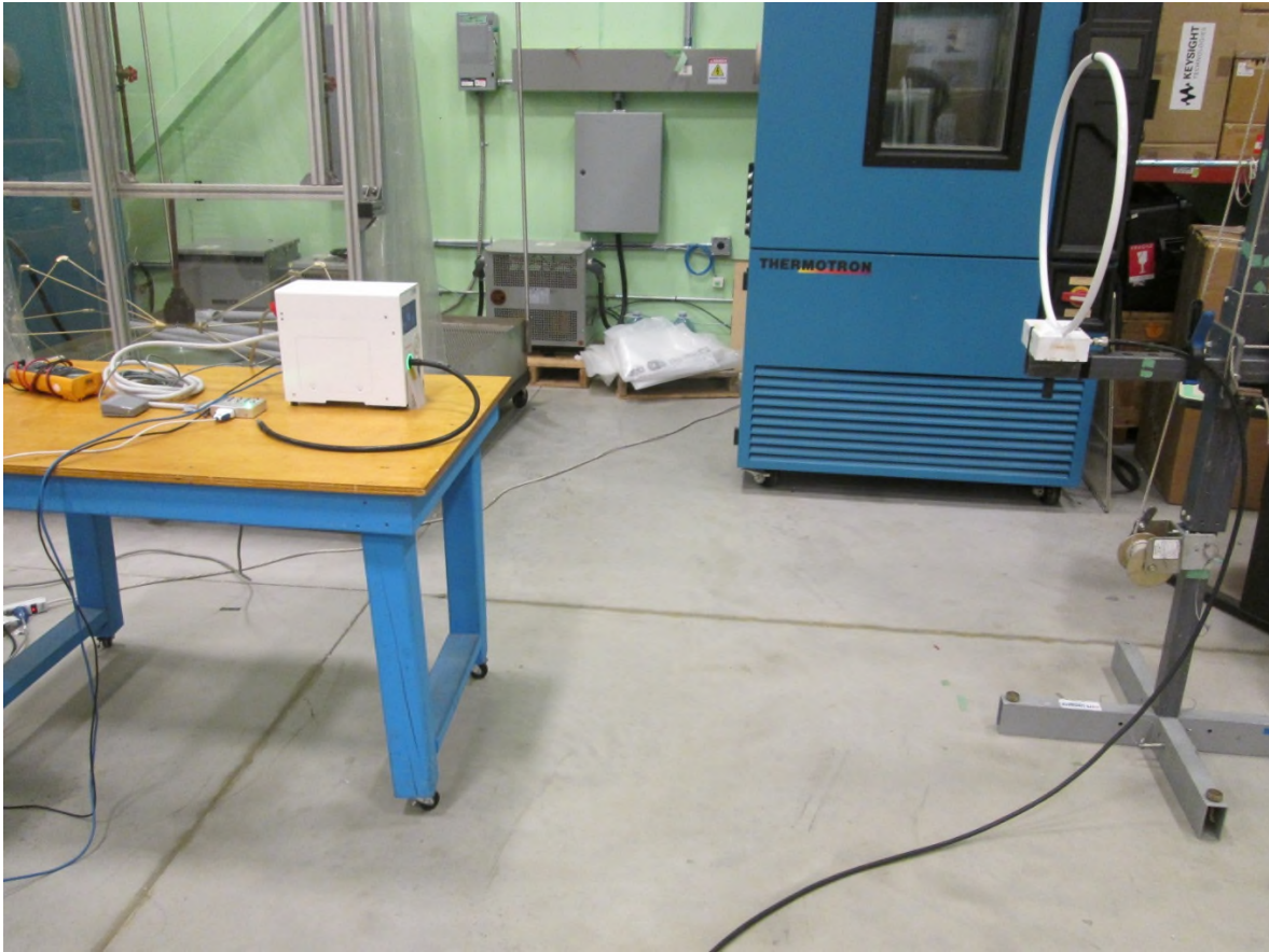
Test setup photo 6 Frequency Stability at Extreme Voltages
