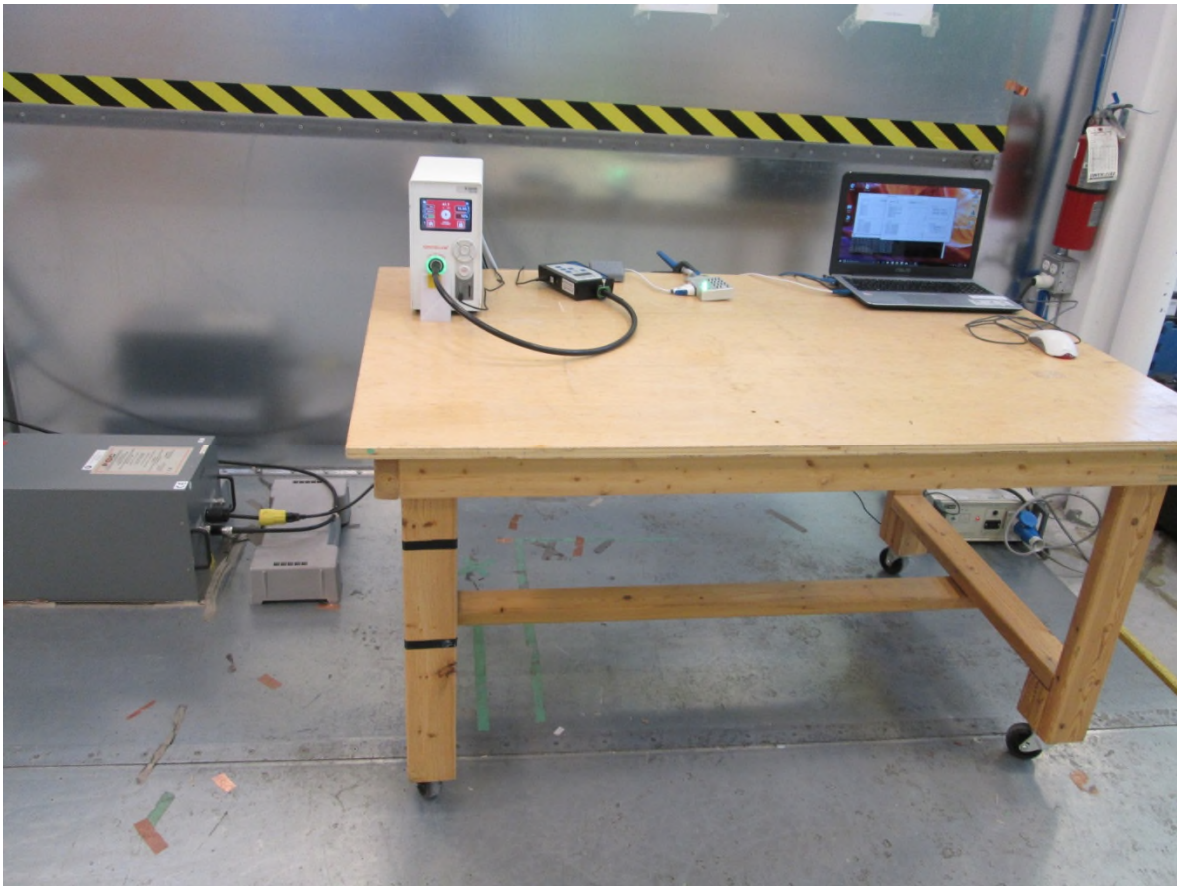
Test setup photo 4 Power line conducted emissions measurements
