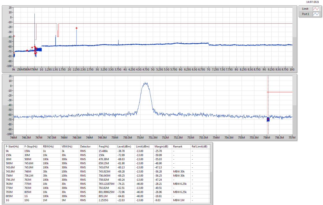
Band 13_NB-IoT_200kHz_Nss1,QPSK_1TX [IM 2.5M] 751.2MHz_QPSK_Tone QPSK
