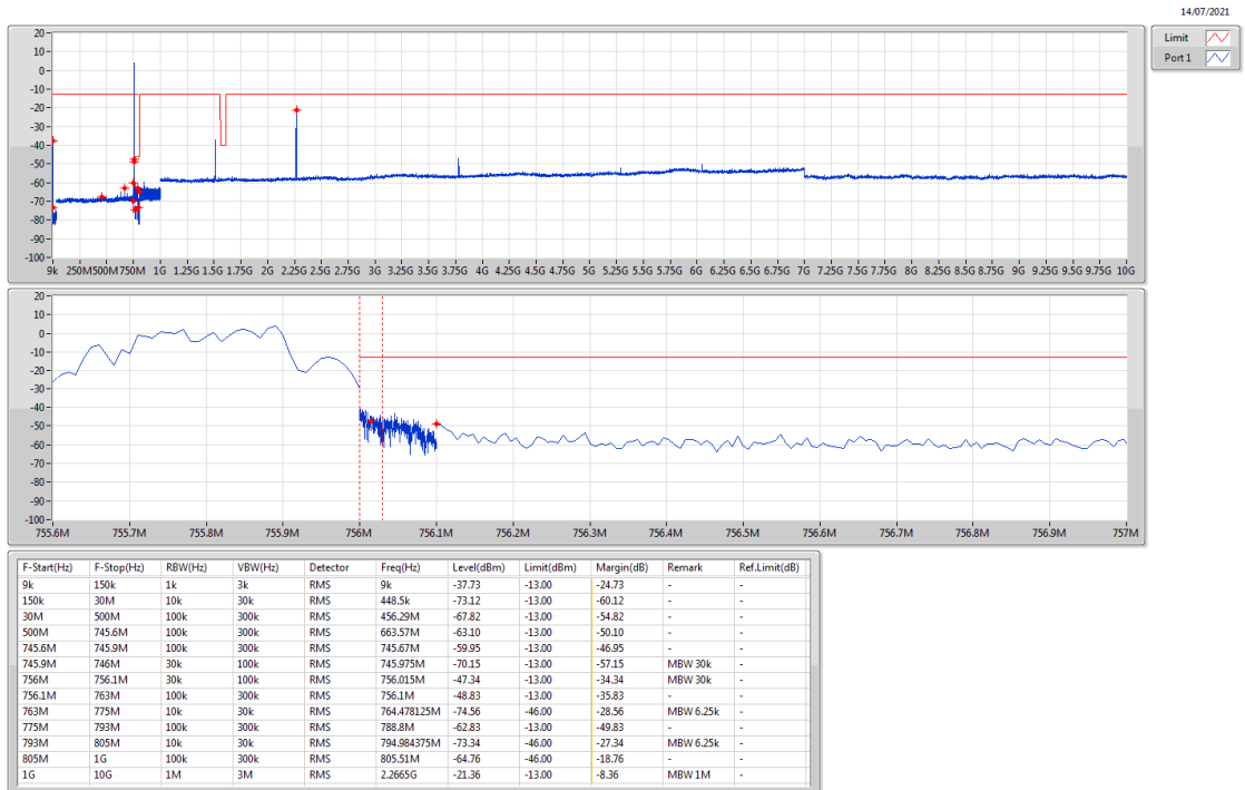
Band 13_NB-IoT_200kHz_Nss1,QPSK_1TX [IM 2.5M] 755.8MHz_QPSK_Tone QPSK
