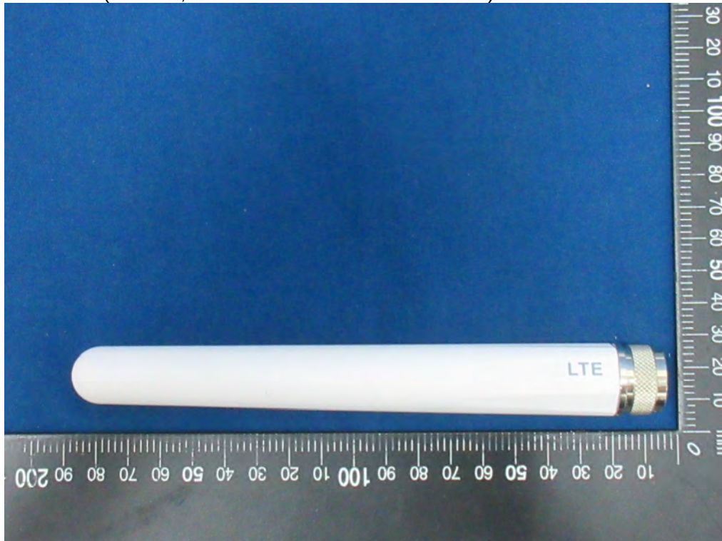
(16) EUT Photo (Antenna, Model No.: JCA225-N)
