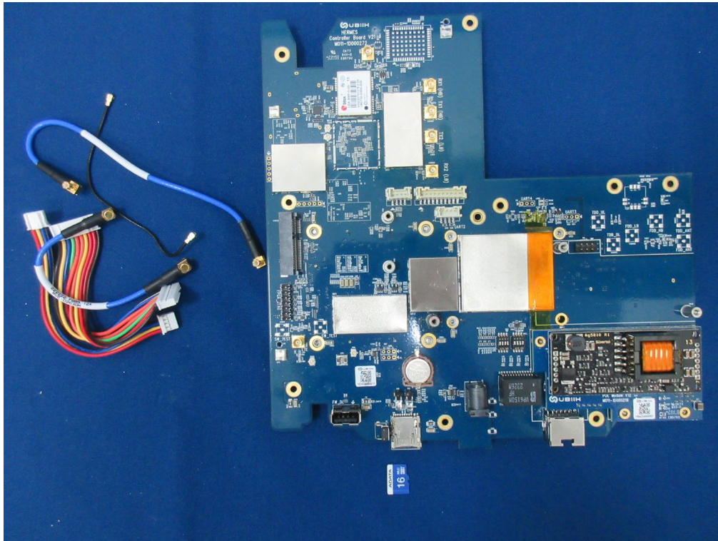
(24) EUT Photo (MicroSD card)
