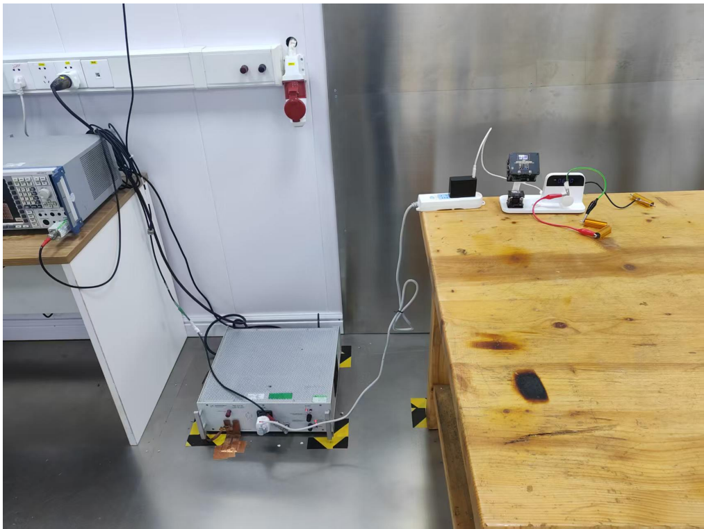
Details of: Conducted emission test view
