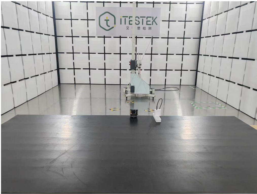
Details of: Radiated emission test (30M-1G Hz) view
