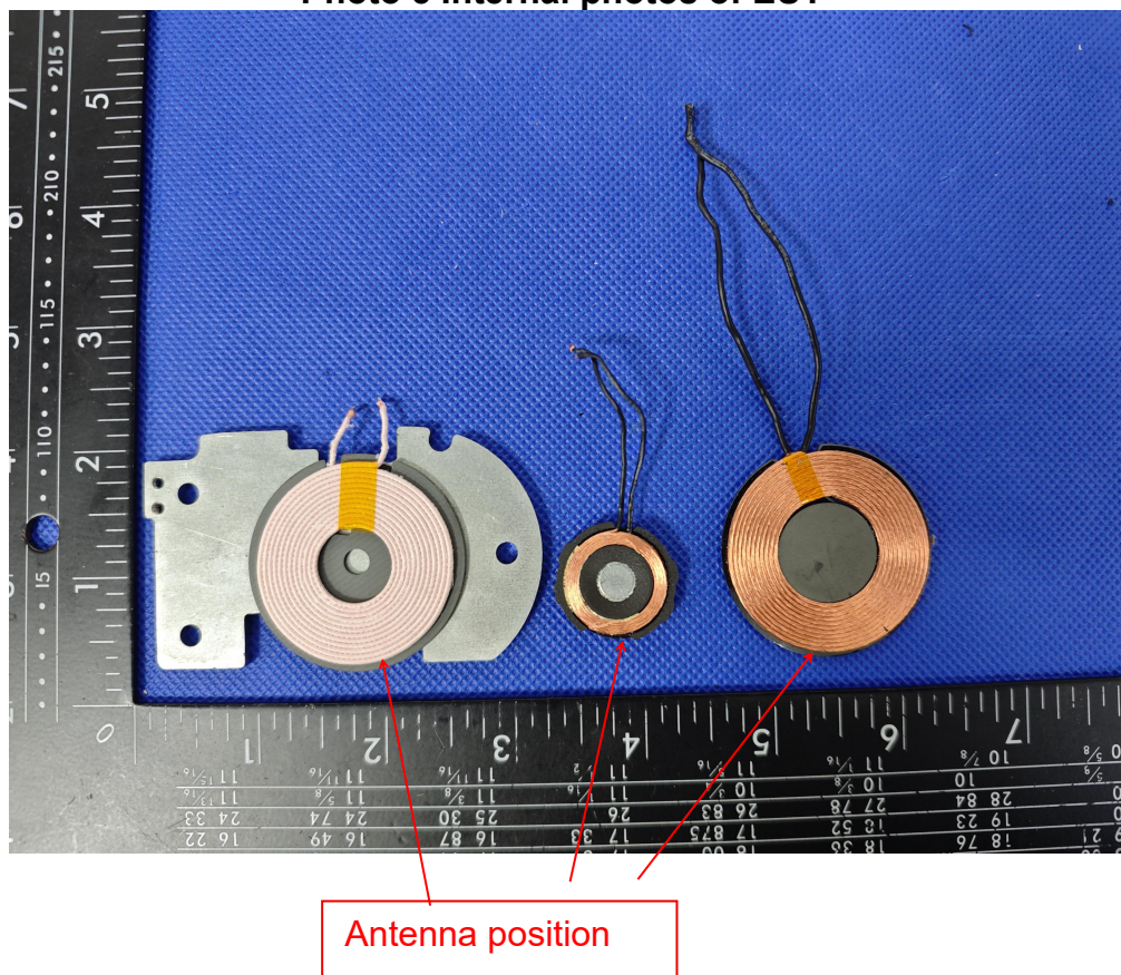
Photo 5 Internal photos of EUT
