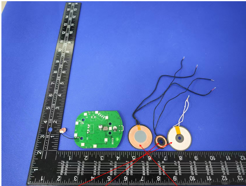
EARPHONE Antenna WATCH Loop Antenna PHONE Loop Antenna
