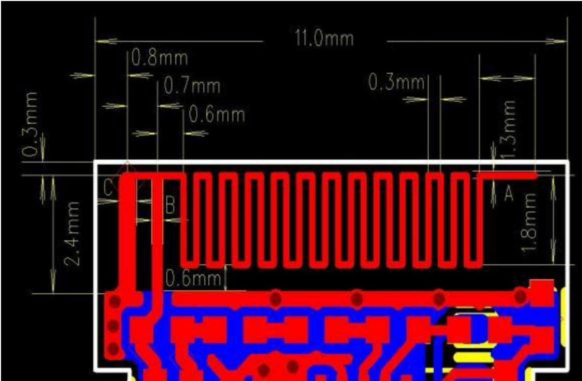
Picture of antenna
