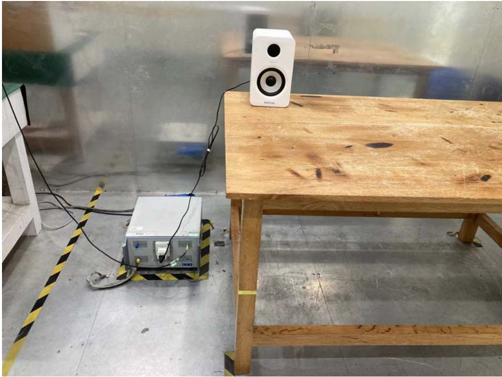
Conducted setup
