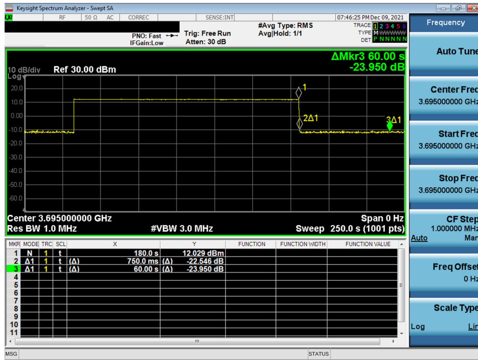
Plot 14. Conducted Measurement - RF transmission stops within 60s of SAS message indicated by Marker 1 (X) (WINNF.FT.C.HBT.3)
