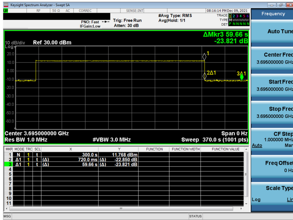
Plot 15. Conducted Measurement - RF transmission stops within 60s of SAS message indicated by Marker 1 (X) (WINNF.FT.C.HBT.4)
