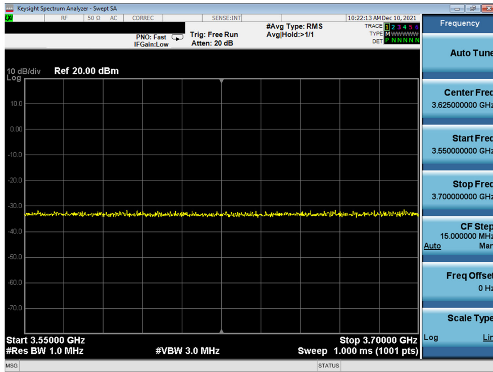
Plot 16. Conducted Measurement – No RF transmission in entire band (WINNF.TT.C.HBT.5)
