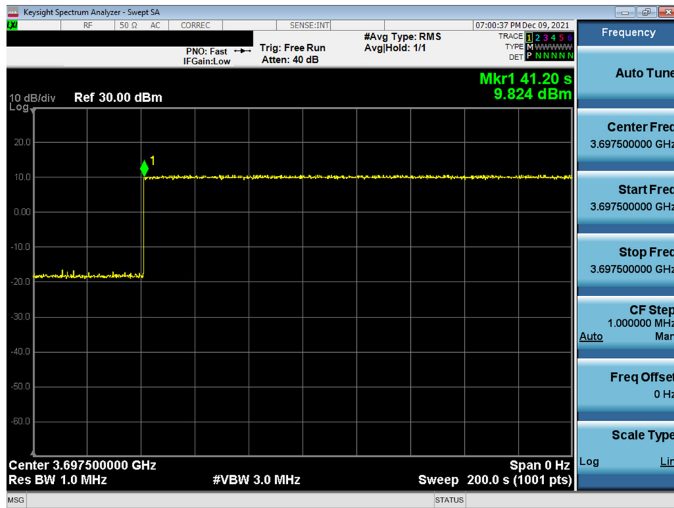
Plot 12. Conducted Measurement - RF transmission after SAS heartbeat response (WINNF.FT.C.HBT.1)
