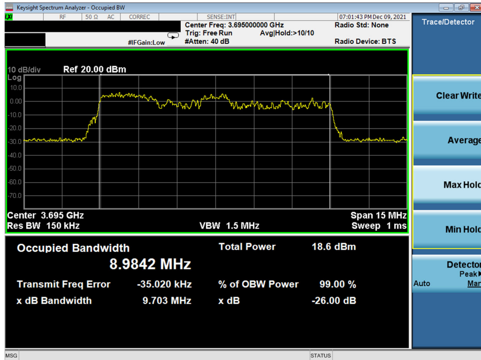
Plot 13. Conducted Measurement Occupied Bandwidth for 10MHz (WINNF.FT.C.HBT.1)
