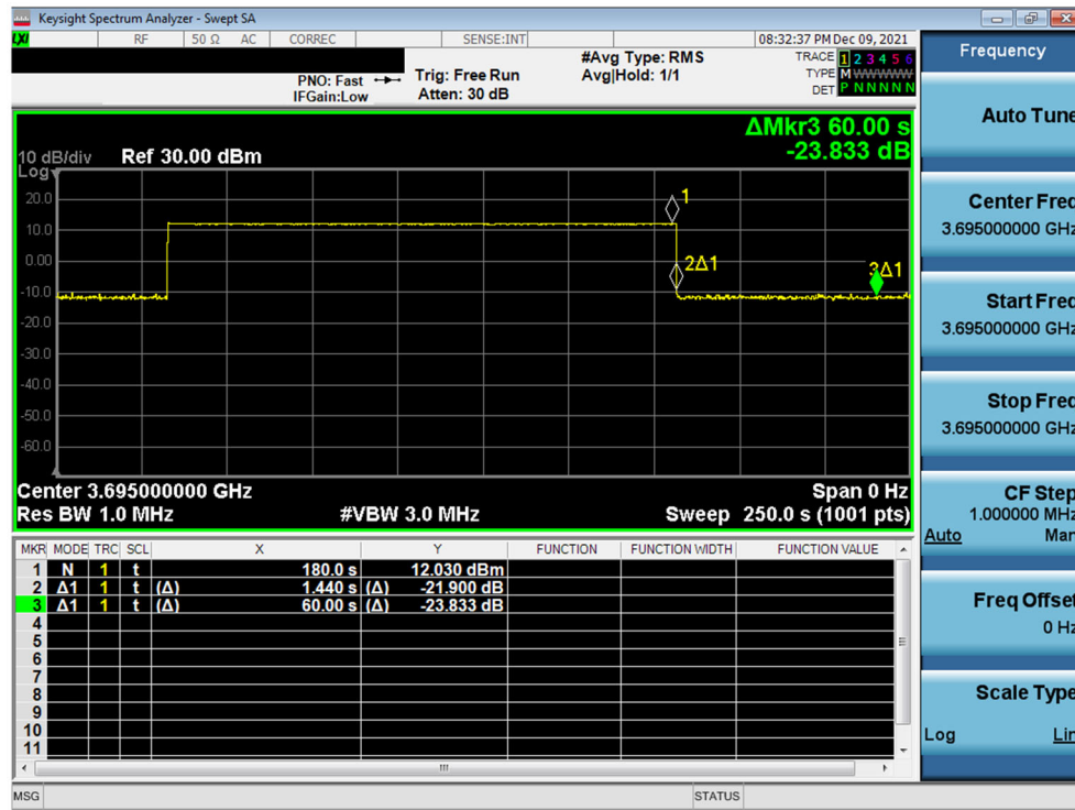
Plot 17. Conducted Measurement - RF transmission stops within 60s of SAS message. The SAS message is indicated by Marker 1 (X) (WINNF.FT.C.HBT.6)
