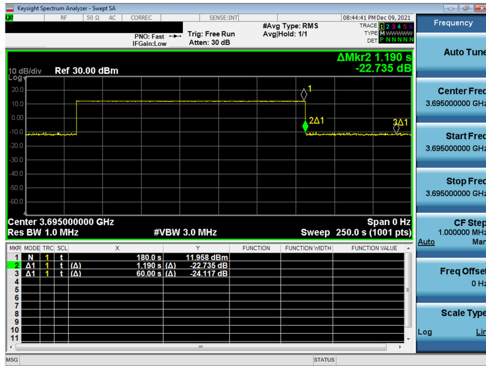
Plot 18. Conducted Measurement - RF transmission stops within 60s of SAS message. The SAS message is indicated by Marker 1 (X) (WINNF.FT.C.HBT.7)
