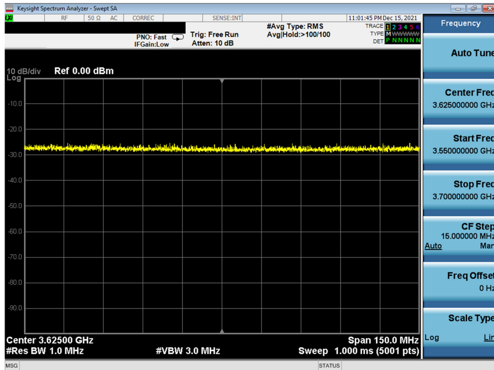
Plot 25. Conducted Measurement – No RF transmission in entire band at anytime (WINNF.FT.C.SCS.2)
