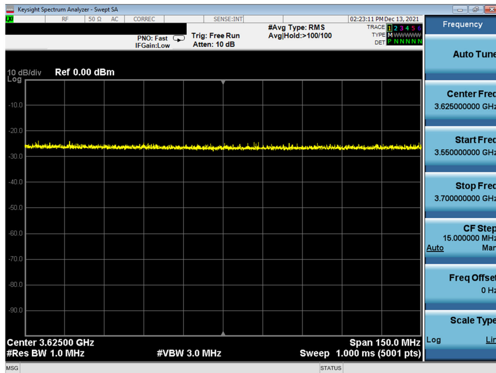
Plot 31. Conducted Measurement – No RF transmission in entire band at anytime (WINNF.FT.C.SCS.5)
