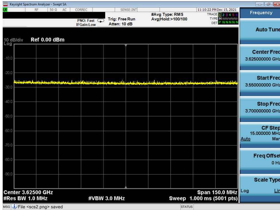
Plot 27. Conducted Measurement – No RF transmission in entire band at anytime (WINNF.FT.C.SCS.3)
