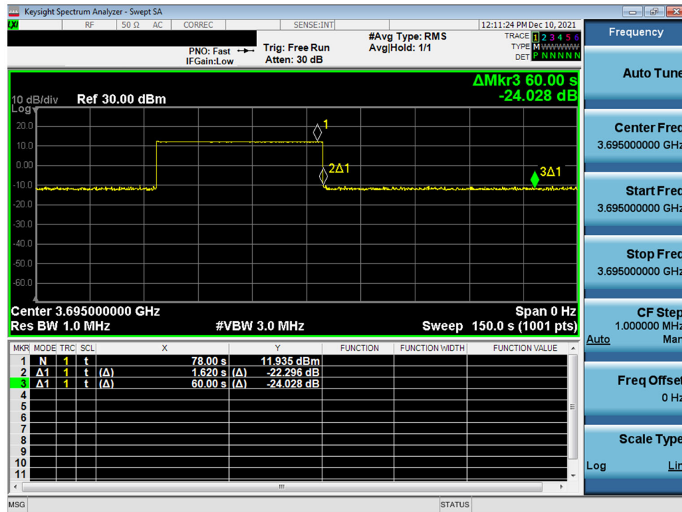
Plot 21. Conducted Measurement - RF transmission stops (WINNF.FT.C.RLQ.1)
