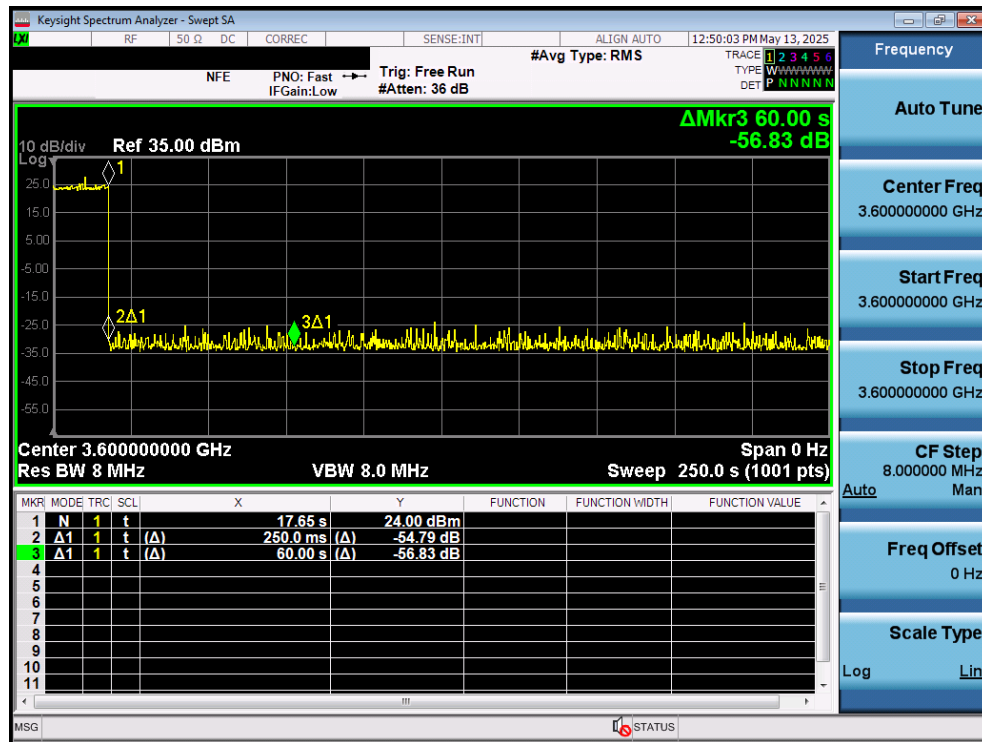
Plot 14. Conducted Measurement – RF transmission ceases with 60s of SAS heartbeat response (WINNF.FT.C.HBT.3)
