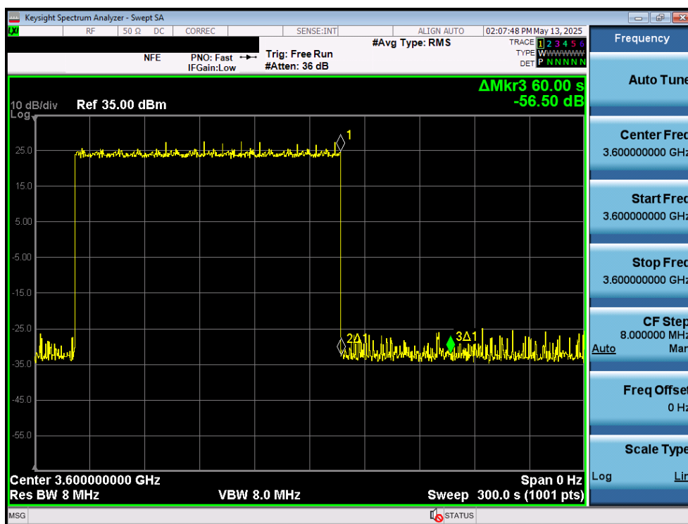
Plot 21. Conducted Measurement – RF Transmission stops within 60s of relinquishment response (WINNF.FT.C.RLQ.1)
