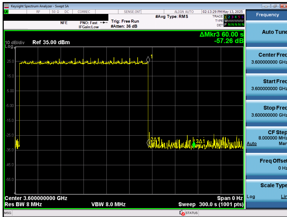
Plot 22. Conducted Measurement – No RF Transmission stops with 60s of deregistration response (WINNF.FT.C.DRG.1)
