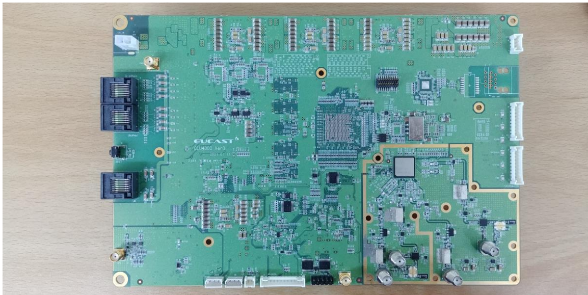
CLU4000_bottom
