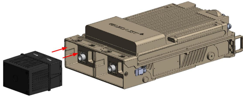
Figure 3. Battery Interface
