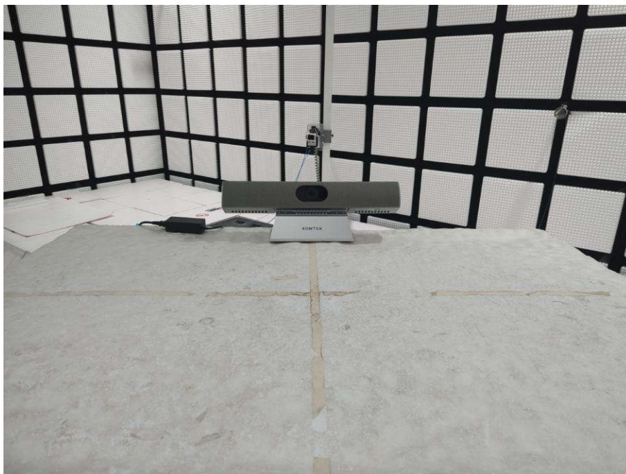
Radiated spurious emission Test Setup-3(18-40 GHz)
