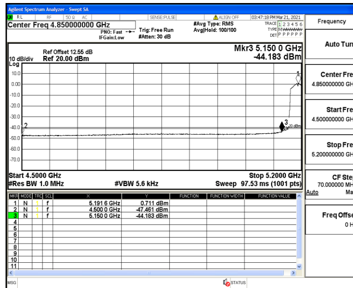
11AC40SISO_Ant1_Low_5190_Peak
