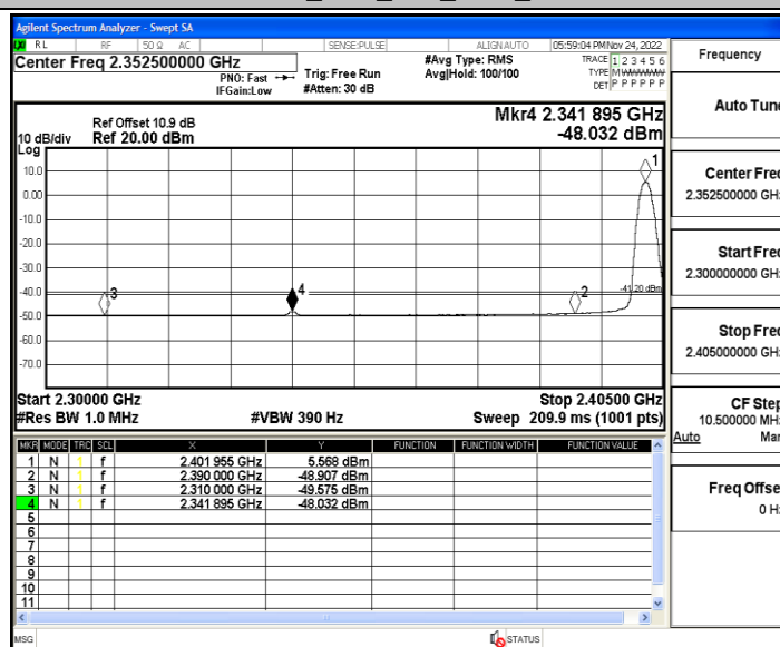
3DH5_Ant2_Low_2402_Peak
