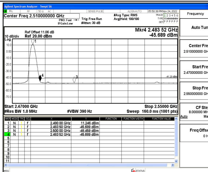
DH5_Ant2_High_2480_Peak
