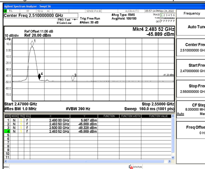
2DH5_Ant2_High_2480_Peak
