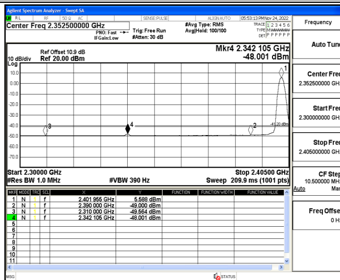
2DH5_Ant2_Low_2402_Peak
