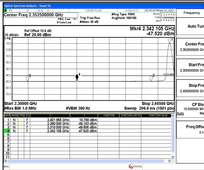
DH5_Ant2_Low_2402_Peak
