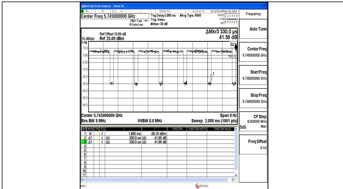
NTNV-11AX20MIMO-Ant2-5745
