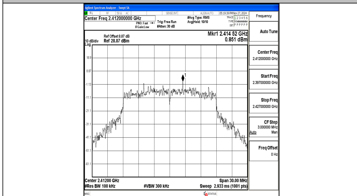
11N20MIMO-Ant2-2412-0~Reference-PASS
