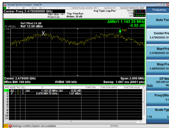
Highest channel
