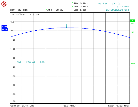
3DH1_2470 3.27dBm
