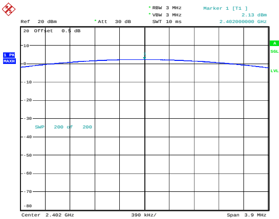
DH1_2402 2.13dBm
