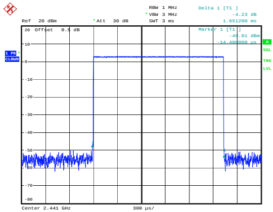
DH3_Hopping 1.651ms
