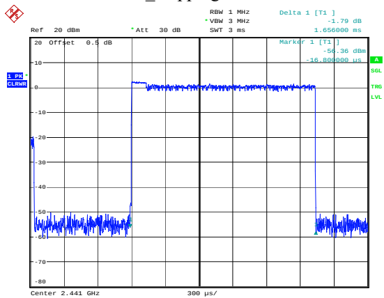
2DH3_Hopping 1.656ms
