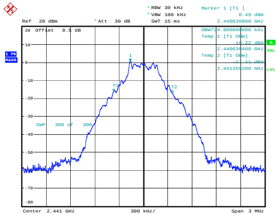
DH1_Middle 0.725MHz
