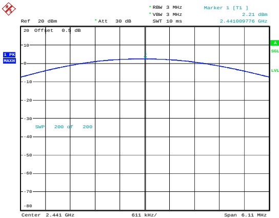
3DH1_2441 2.21dBm
