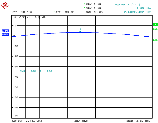
DH1_2440 2.95dBm
