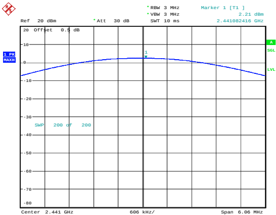
2DH1_2441 2.21dBm
