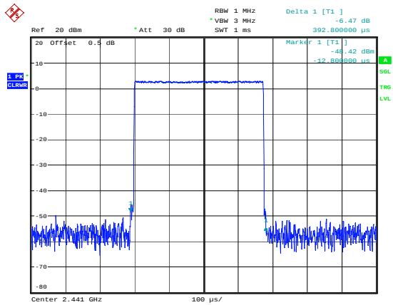
DH1_Hopping 0.393ms
