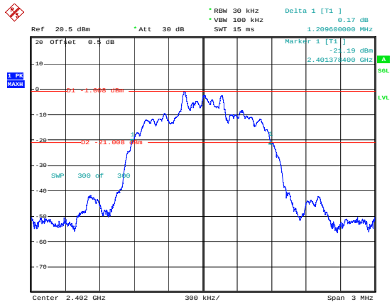
2DH1_Low 1.210MHz
