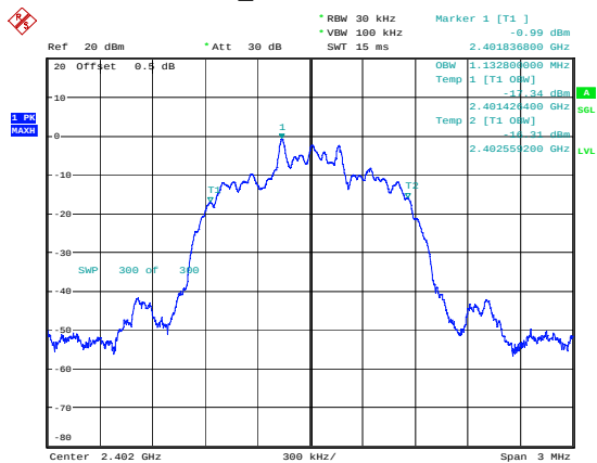
2DH1_Low 1.133MHz
