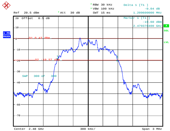
2DH1_High 1.210MHz
