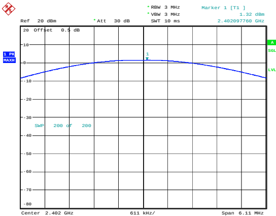
3DH1_2402 1.32dBm
