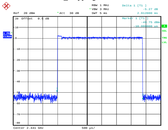
2DH5_Hopping 2.912ms
