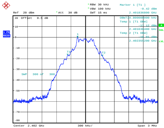
DH1_Low 0.725MHz
