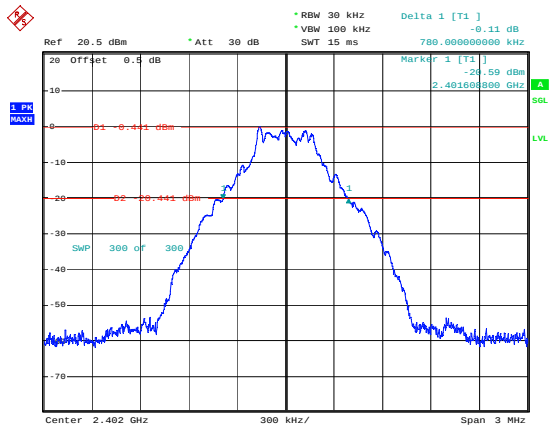
DH1_Low 0.780MHz
