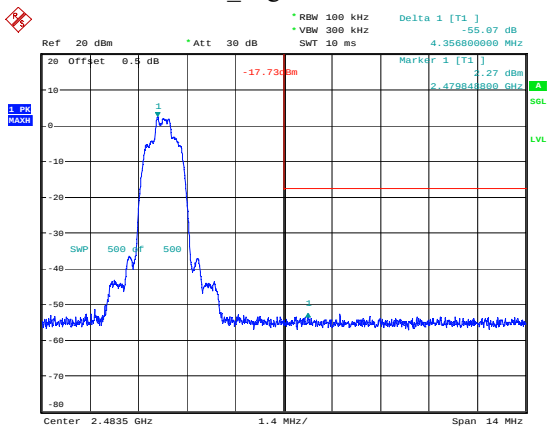
2DH1_High 55.07dB
