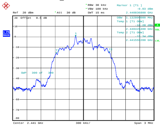
2DH1_Middle 1.133MHz
