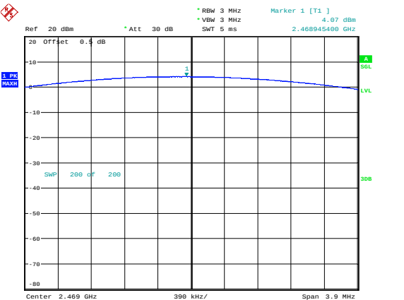
DH1_2469 4.07dBm
