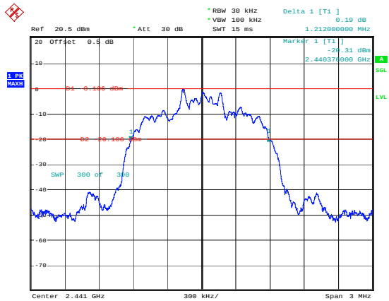
2DH1_Middle 1.212MHz
