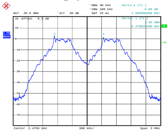
DH1_High 1.001MHz
