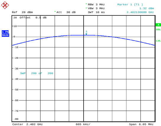
2DH1_2402 1.32dBm
