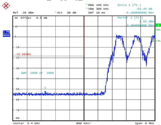
DH1_Hopping_Lower 53.44dB
