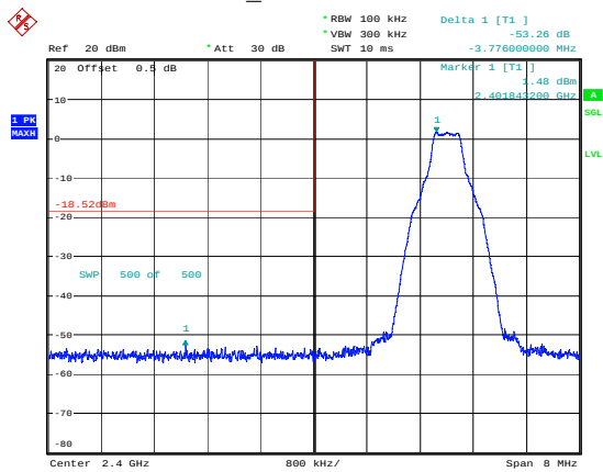
DH1_Low 53.26dB
