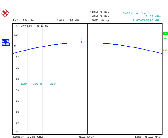
3DH1_2480 2.68dBm
