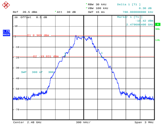
DH1_High 0.780MHz
