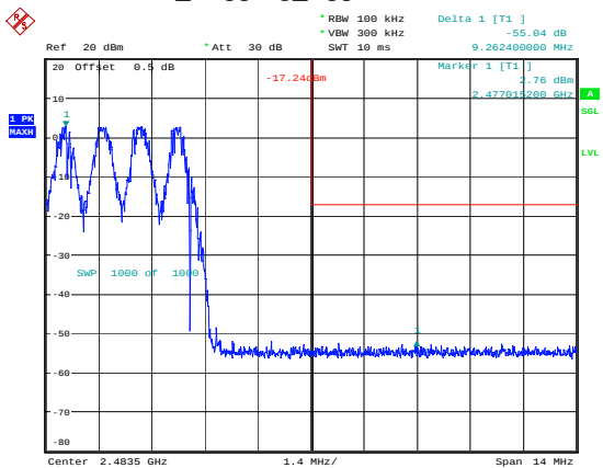
DH1_Hopping_Upper 55.04dB
