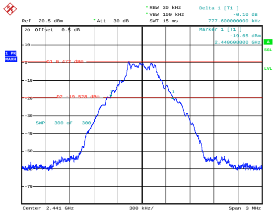
DH1_Middle 0.778MHz
