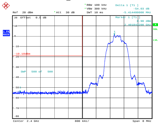
2DH1_Low 54.03dB
