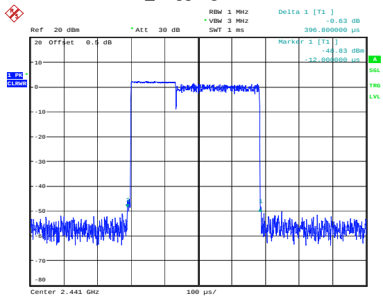
2DH1_Hopping 0.397ms
