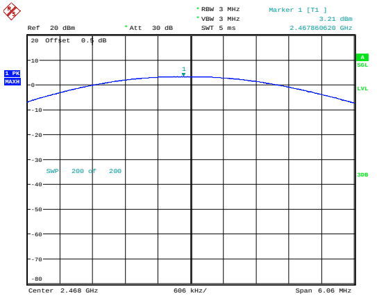
2DH1_2468 3.21dBm
