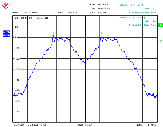
DH1_Middle 1.001MHz
