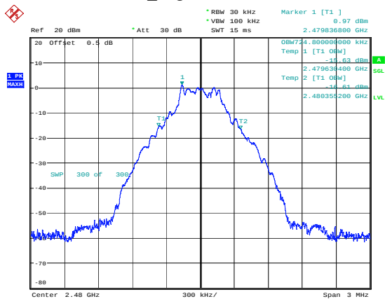
DH1_High 0.725MHz
