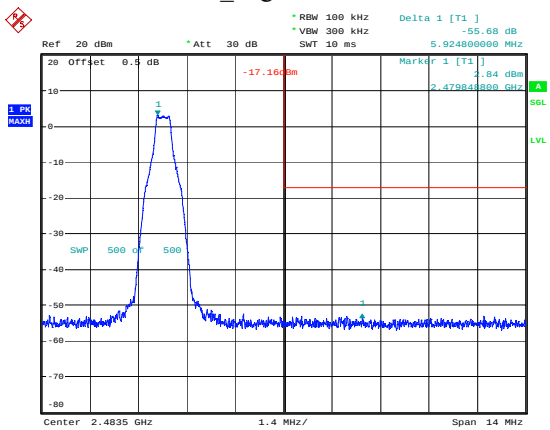
DH1_High 55.68dB
