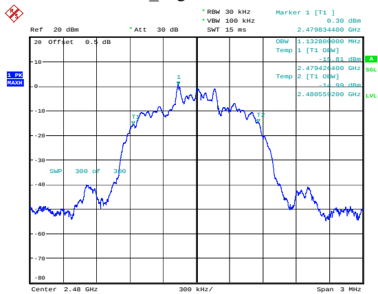
2DH1_High 1.133MHz
