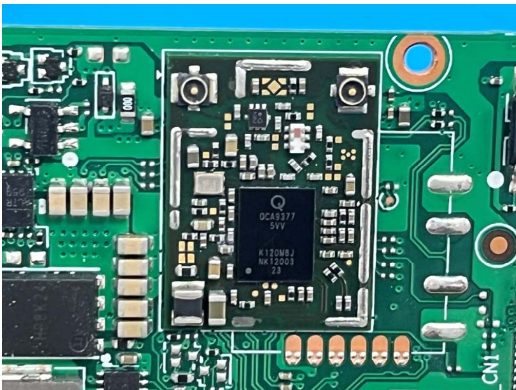
RF Module unshielded
