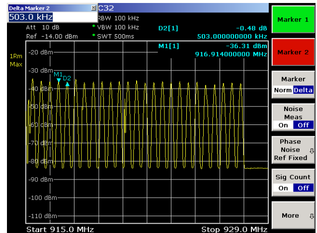
Plot # 5. Hopping channels separation
