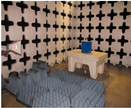
Radiated emissions test set up above 1GHz. Antenna 2 test
