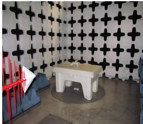
Radiated emissions test set up in 30MHz- 1GHz frequency range
